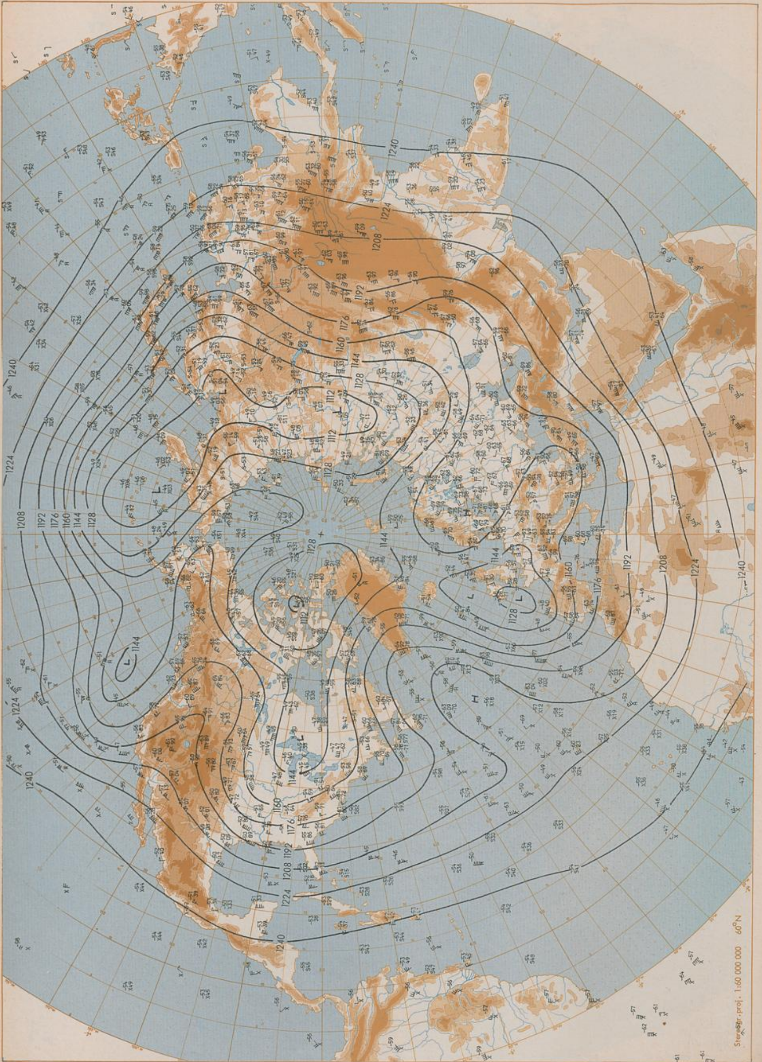
200 hPa 00 UTC
