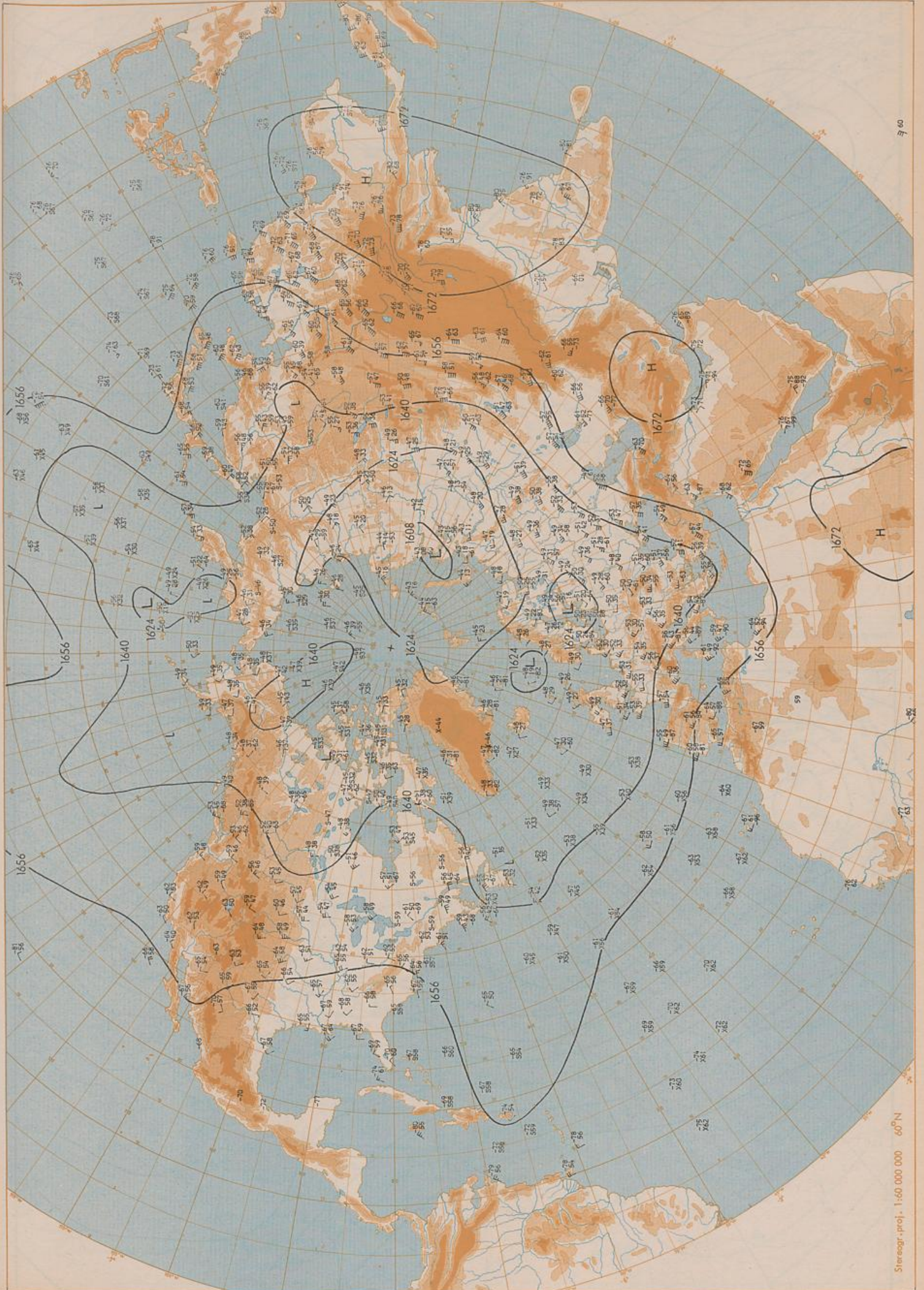
100 hPa 00 UTC
