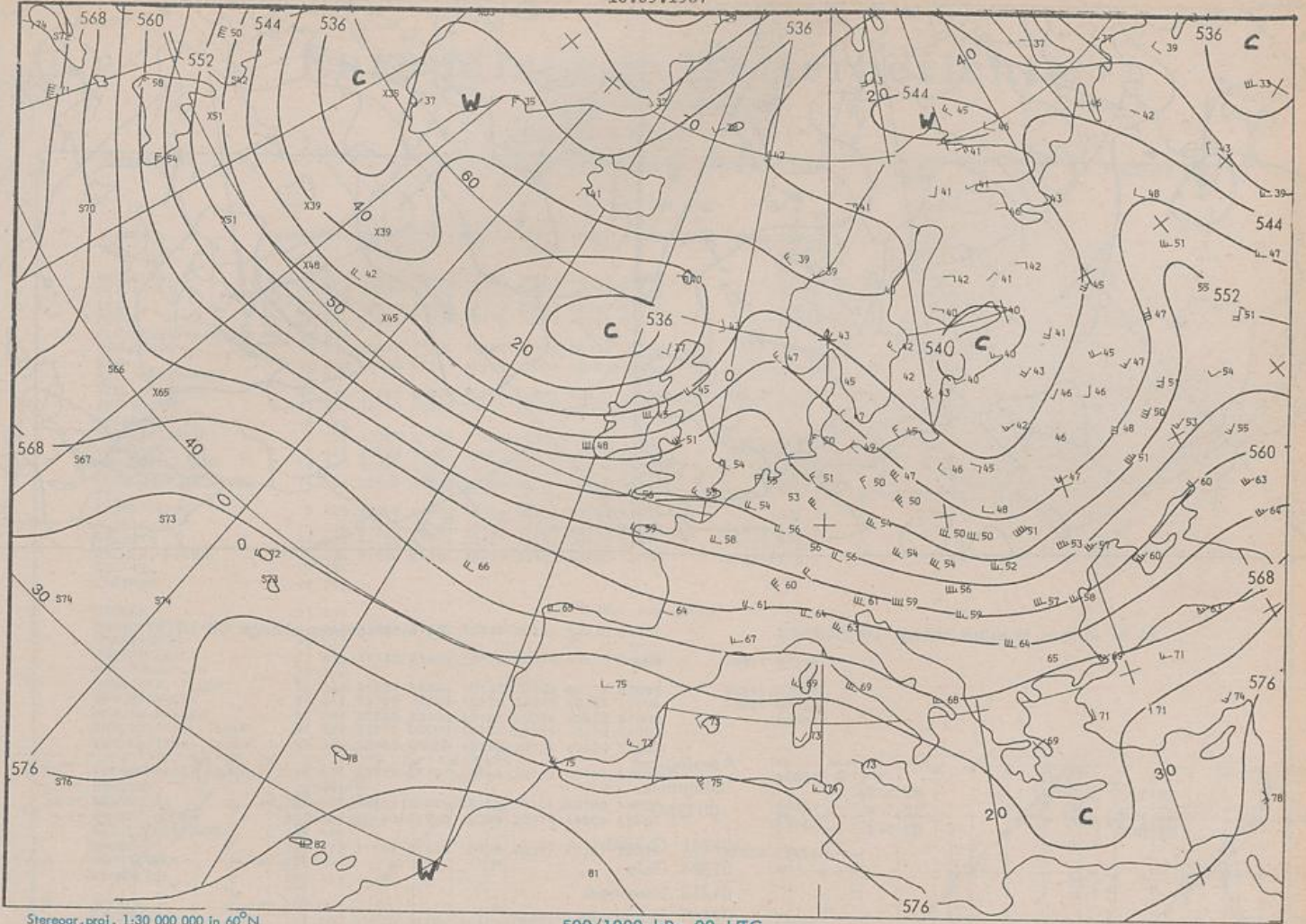
500/1000 hPa 00 UTC
