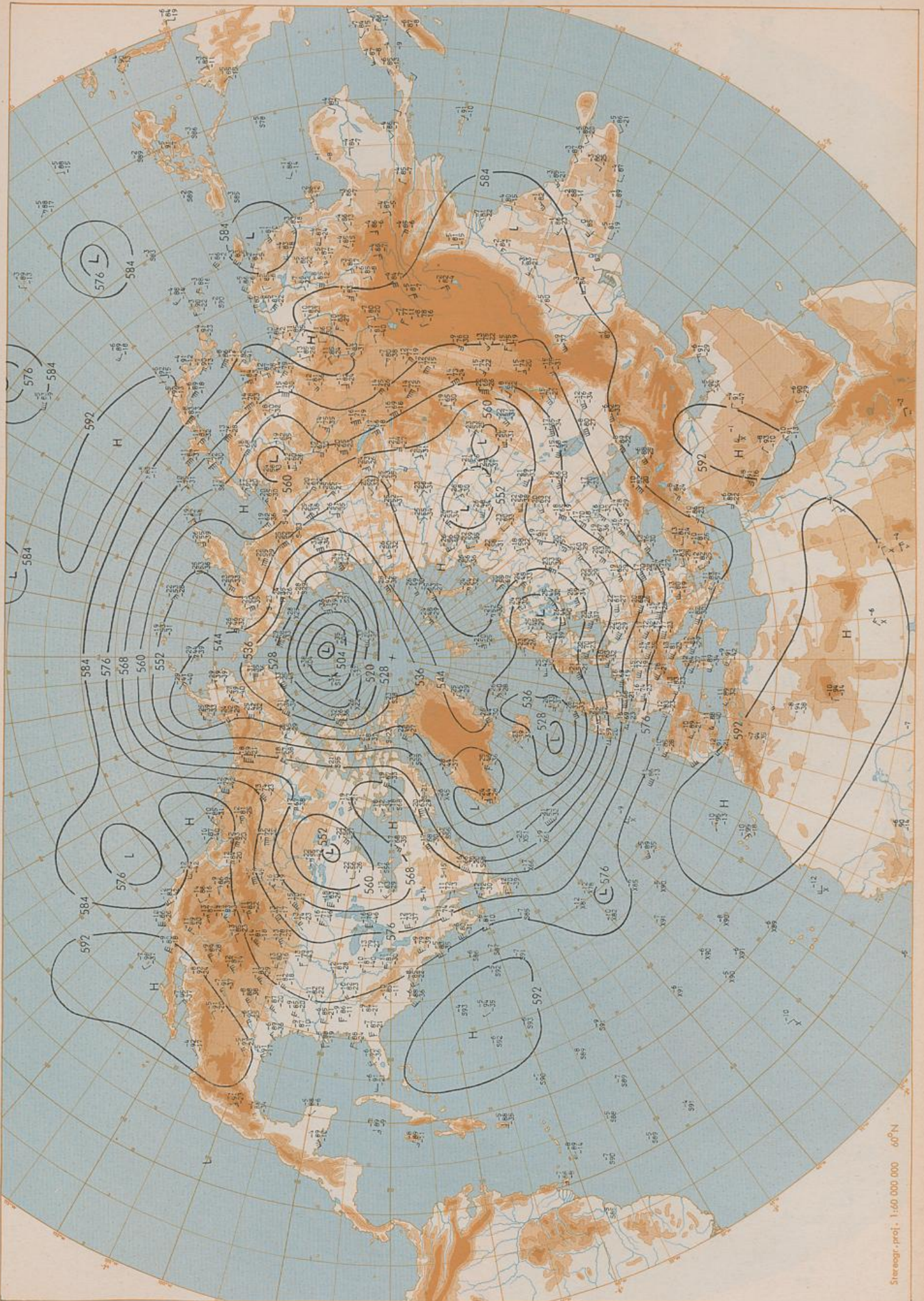
500 hPa 00 UTC
