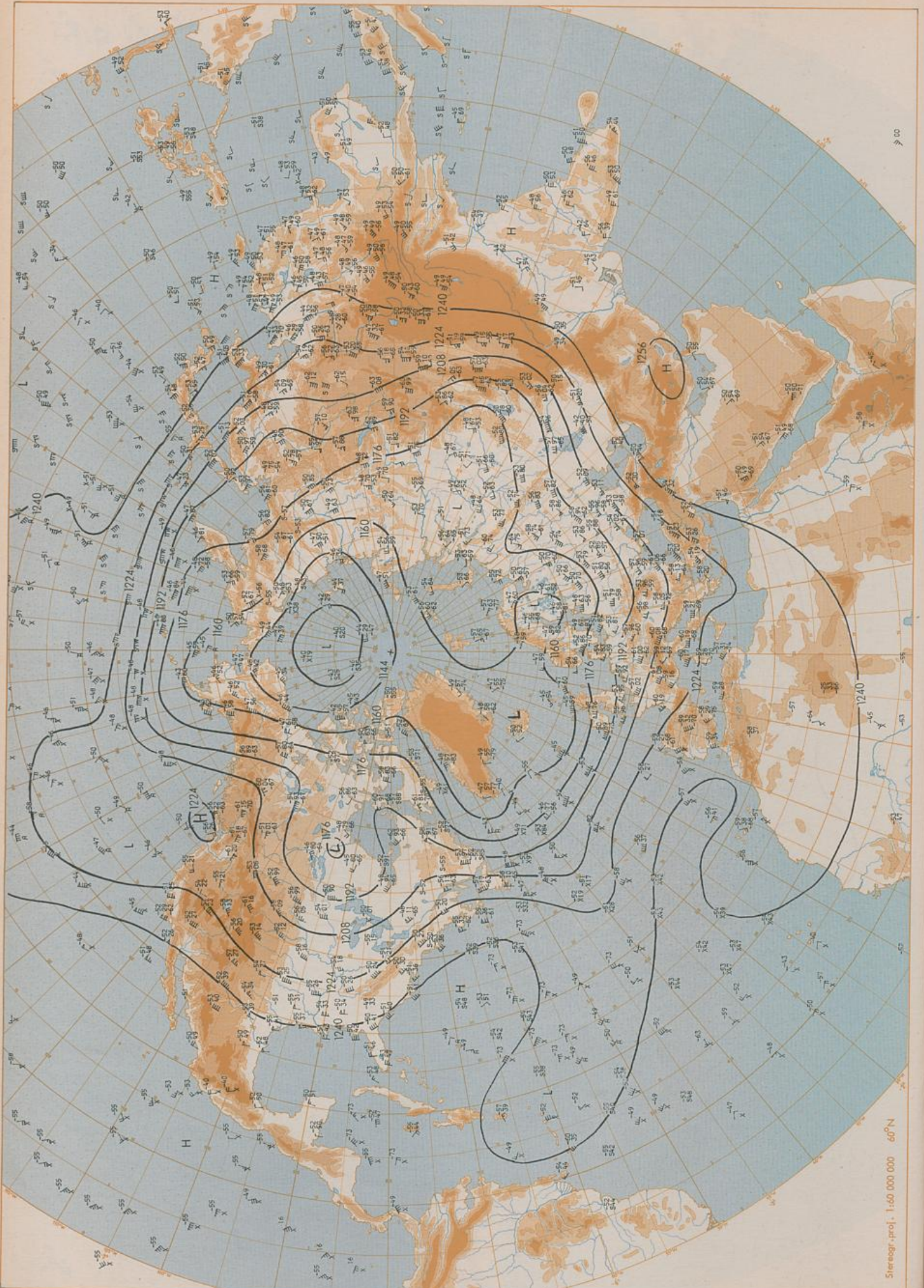
200 hPa 00 UTC
