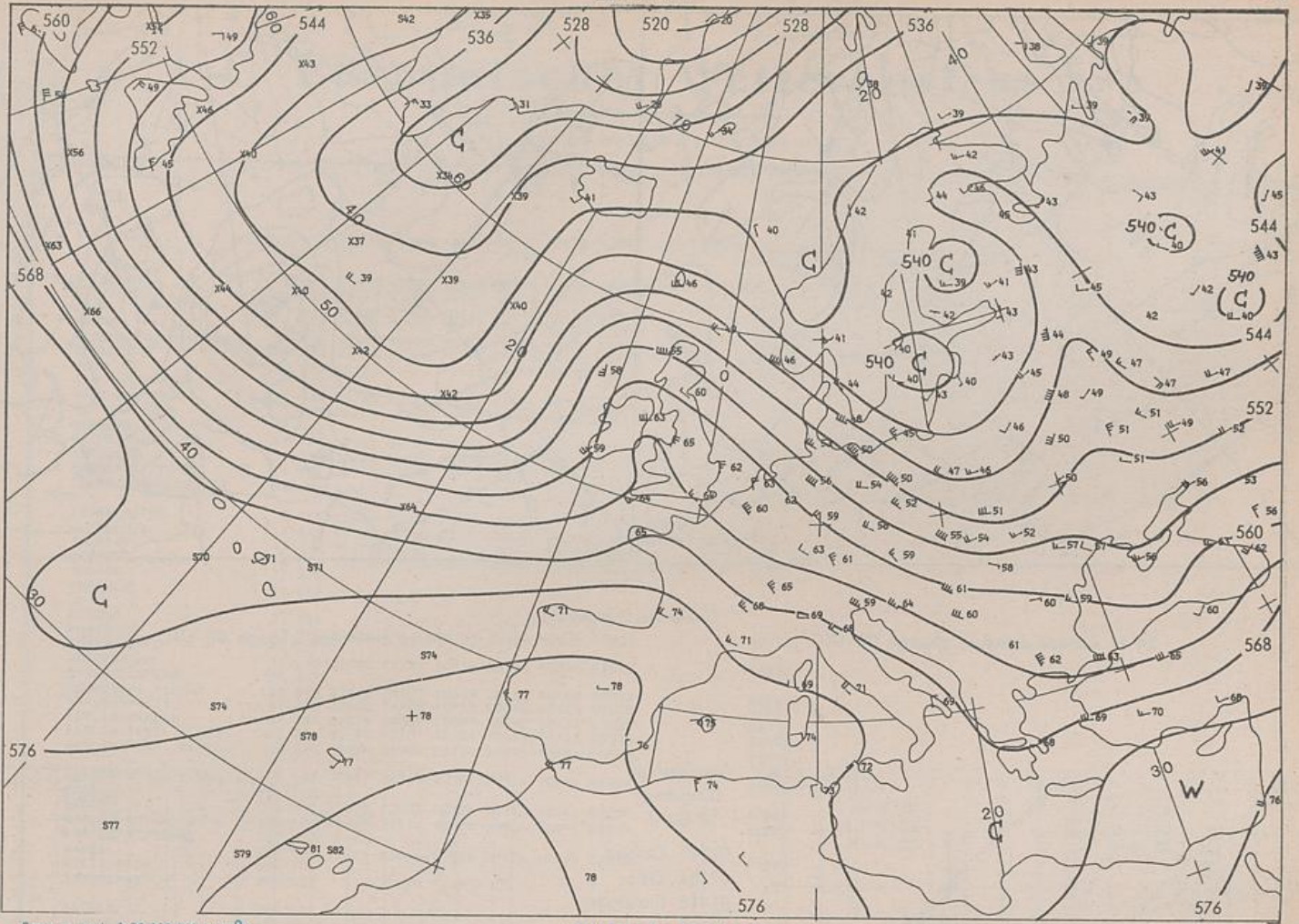
500/1000 hPa 00 UTC
