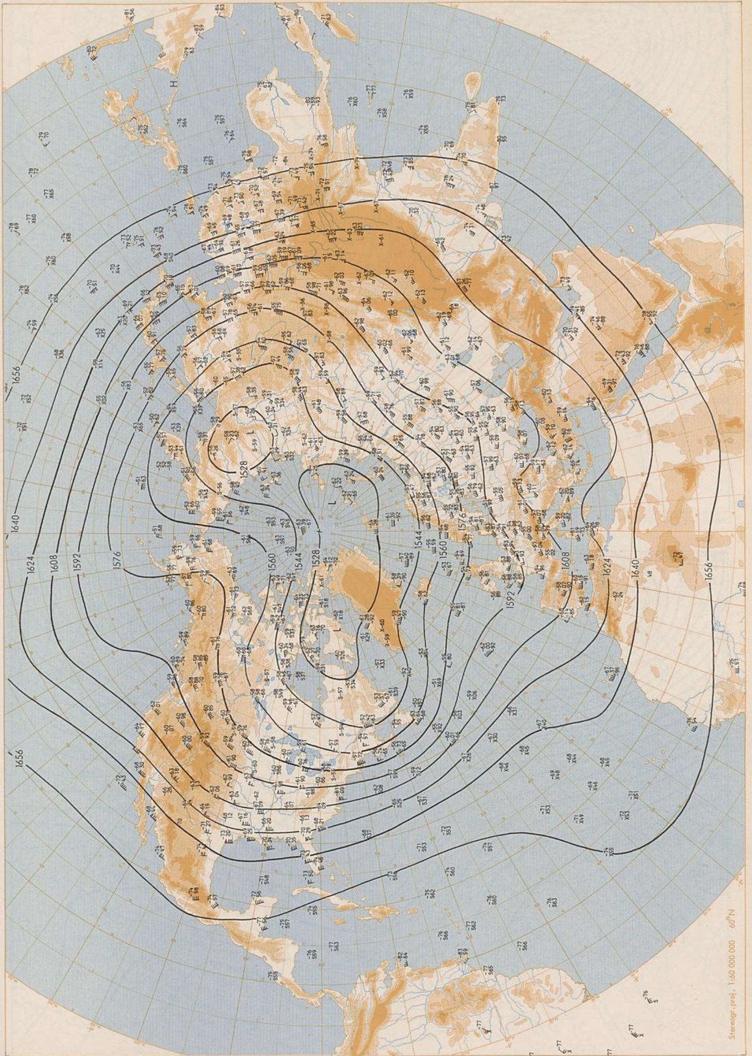
100 hPa 00 UTC
