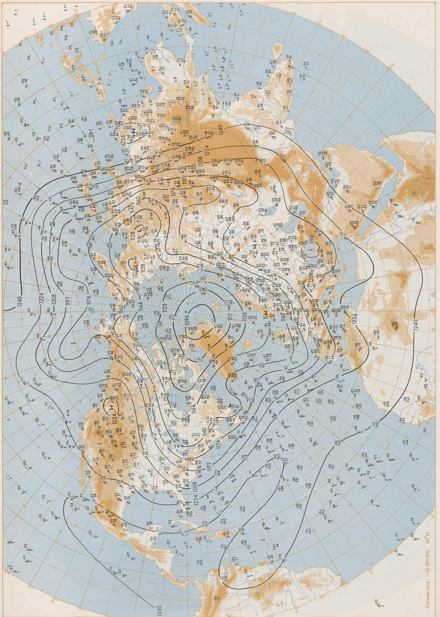
200 hPa 00 UTC
