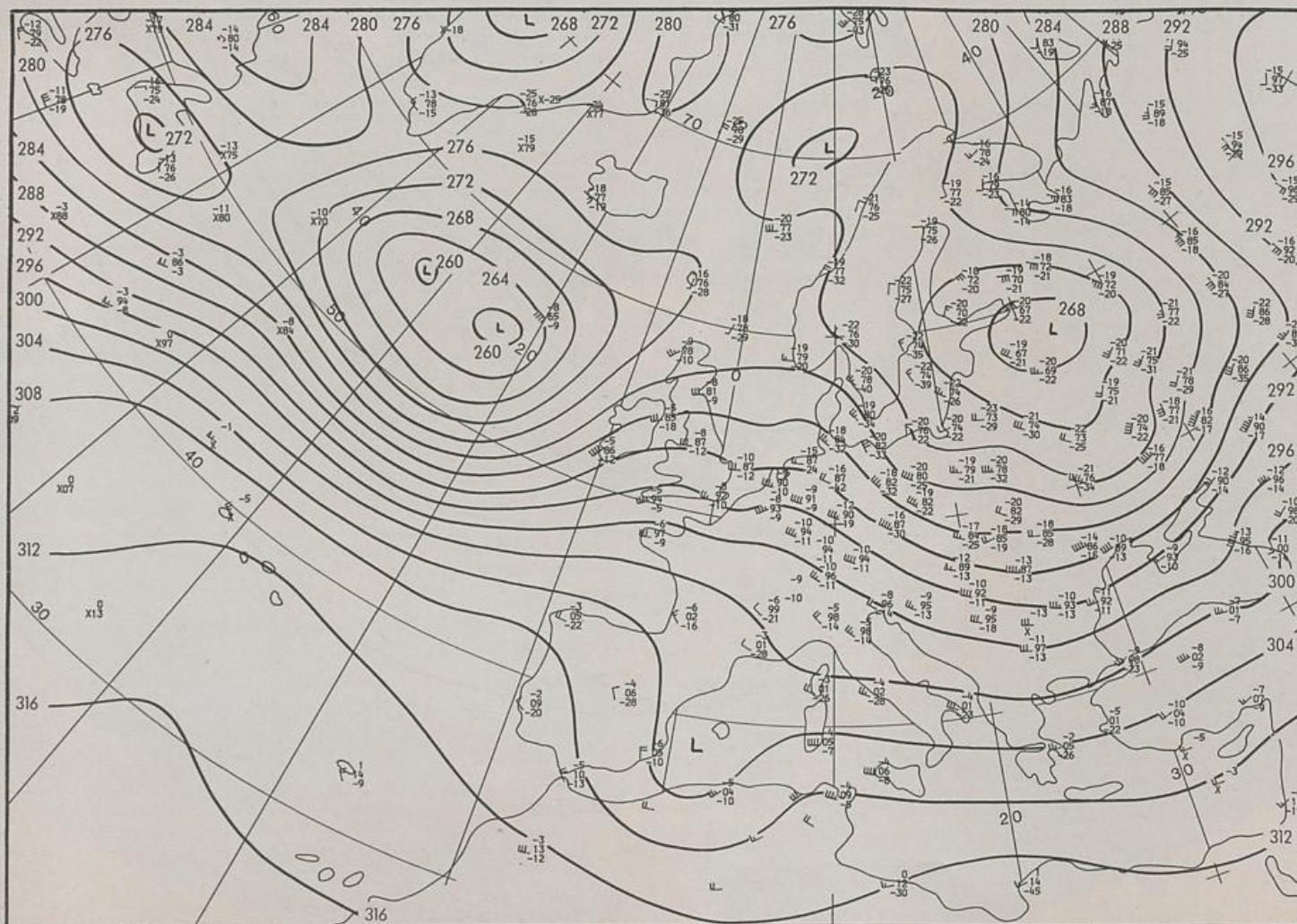
700 hPa 00 UTC
