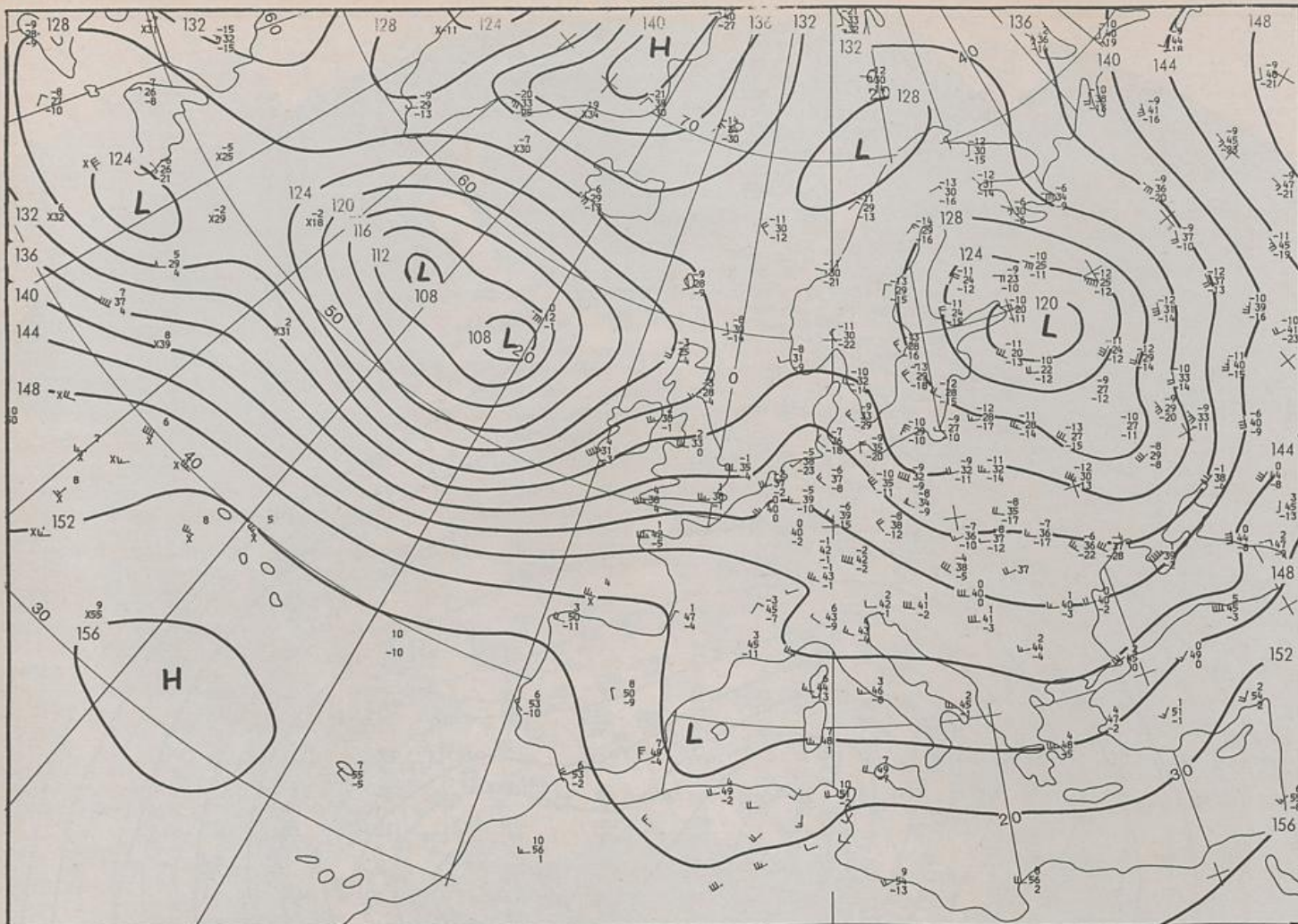
850 hPa 00 UTC
