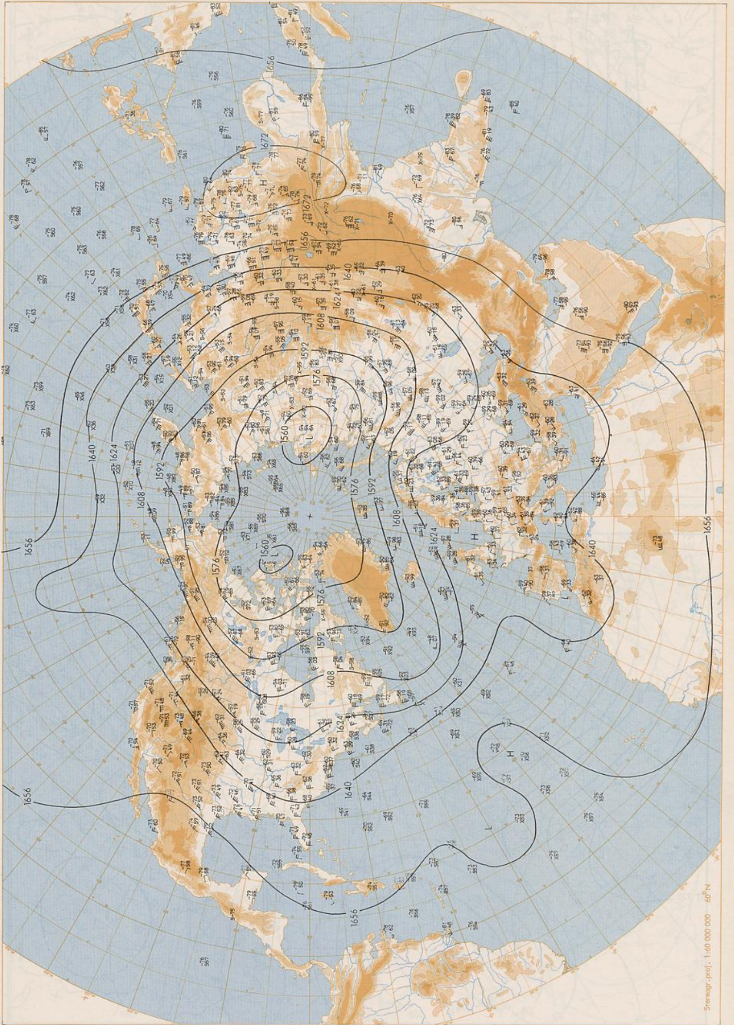
100 hPa 00 UTC
