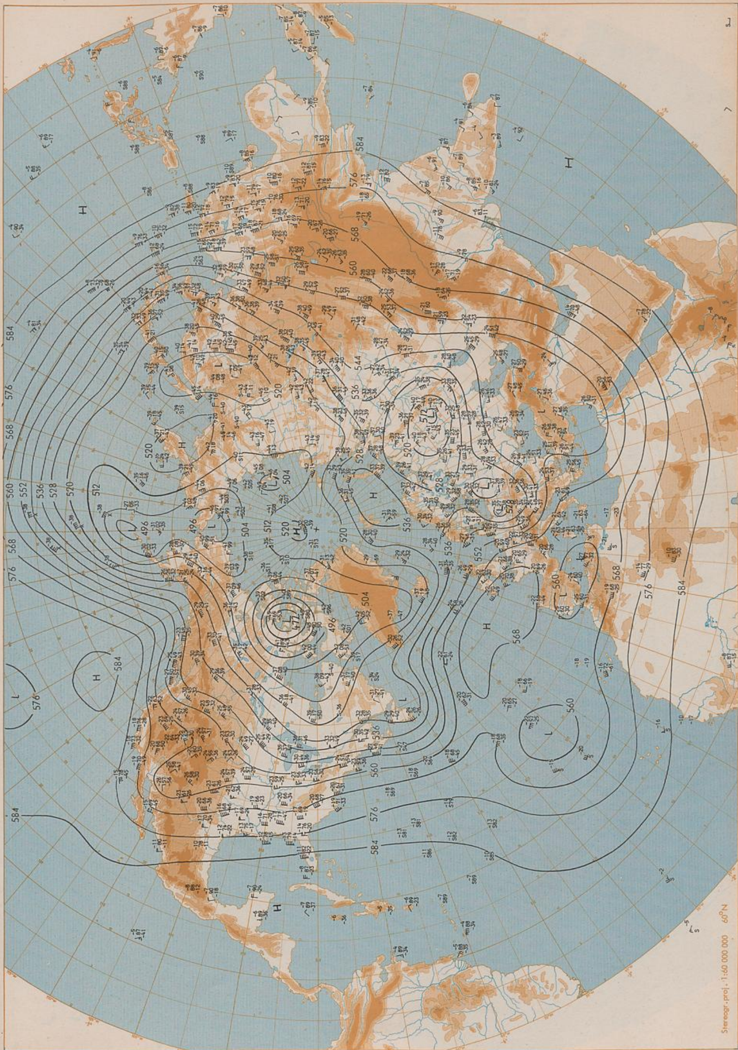
500 hPa 00 UTC
