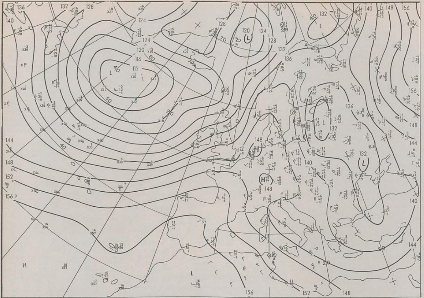
850 hPa 00 UTC
