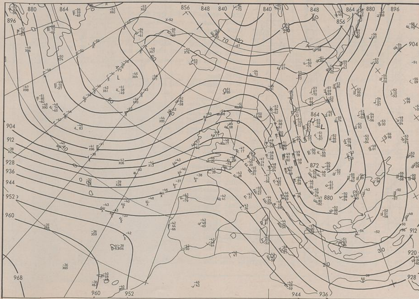
300 hPa 00 UTC
