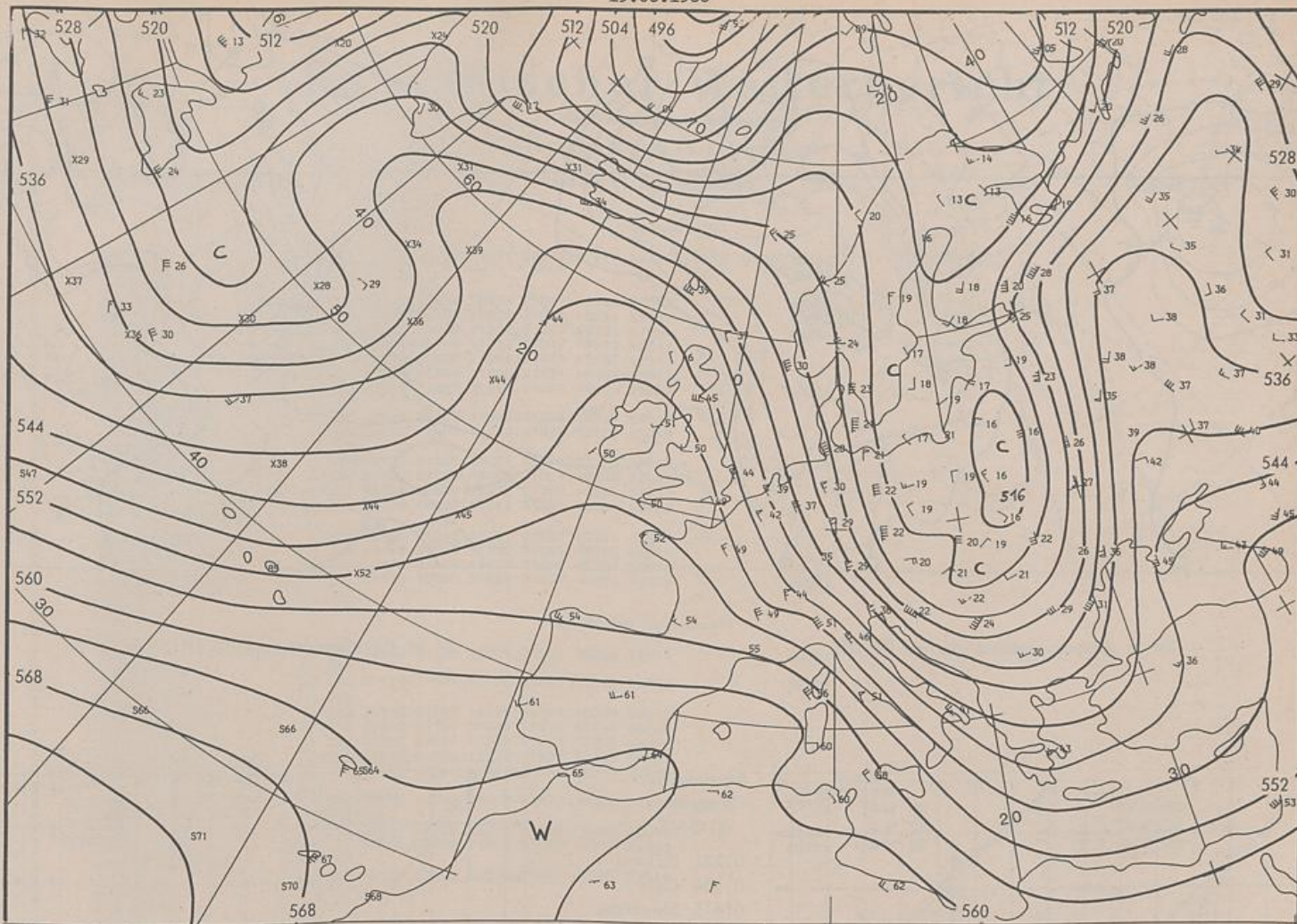
500/1000 hPa 00 UTC
