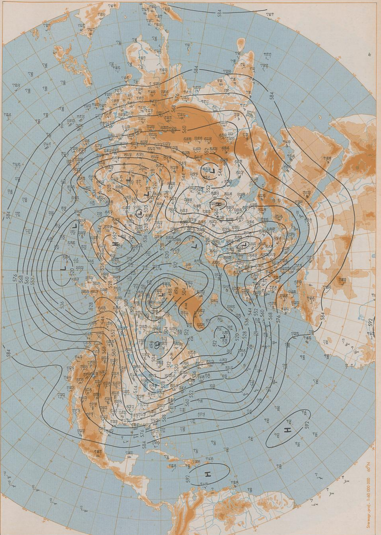
500 hPa 00 UTC
