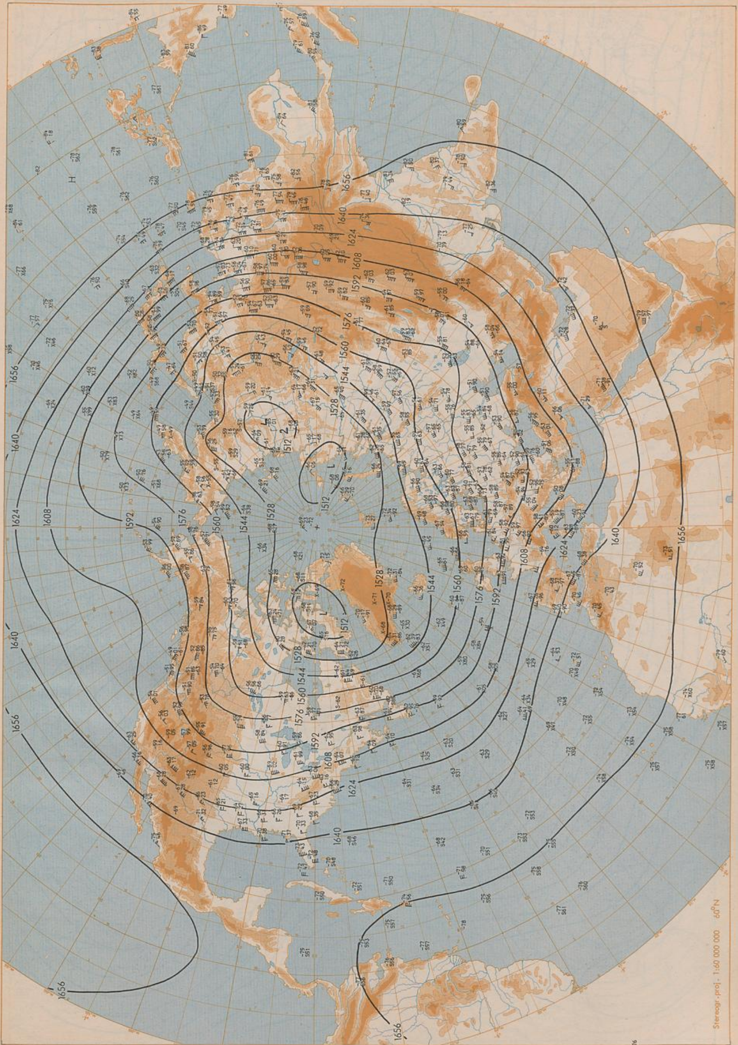
100 hPa 00 UTC
