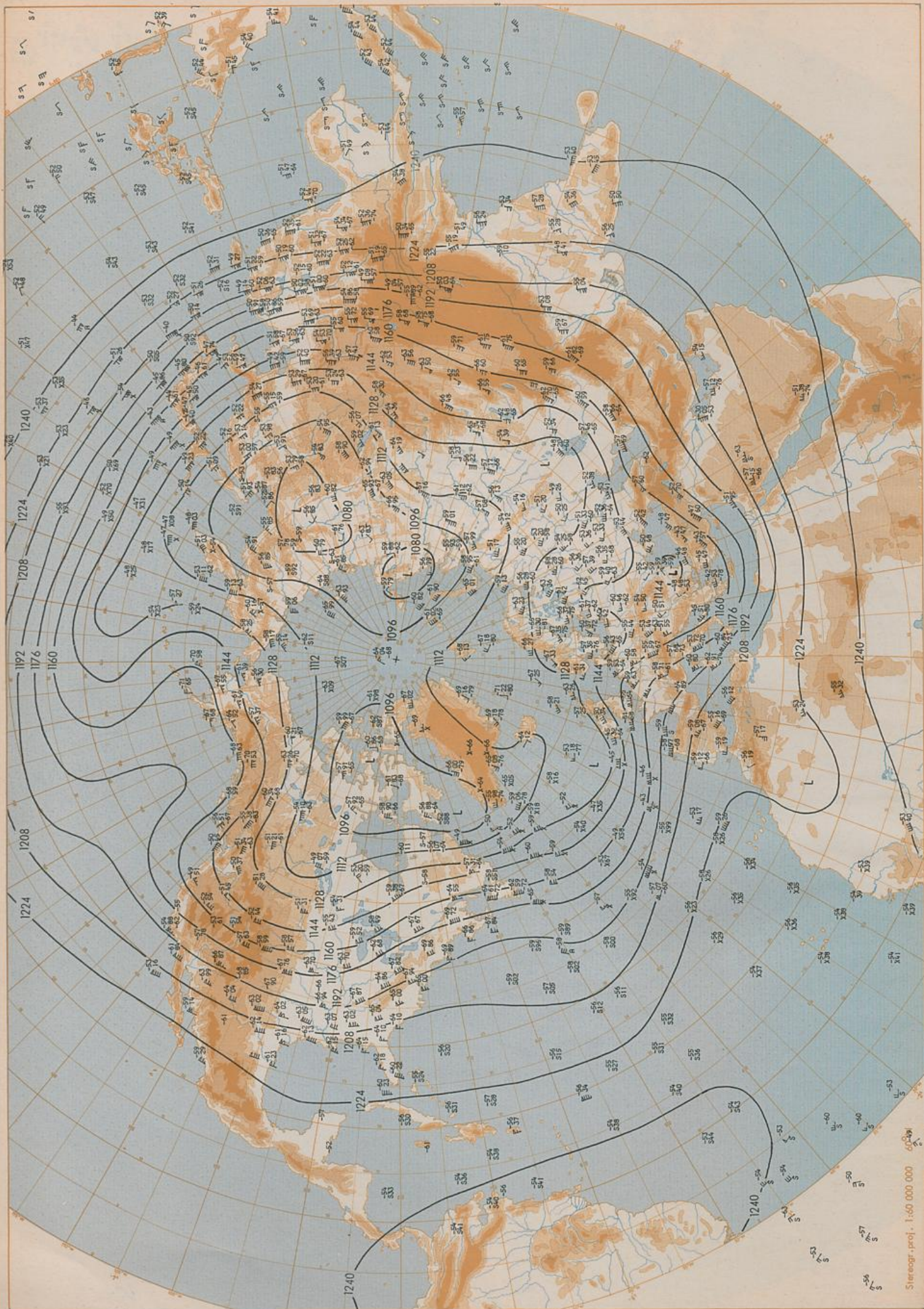
200 hPa 00 UTC
