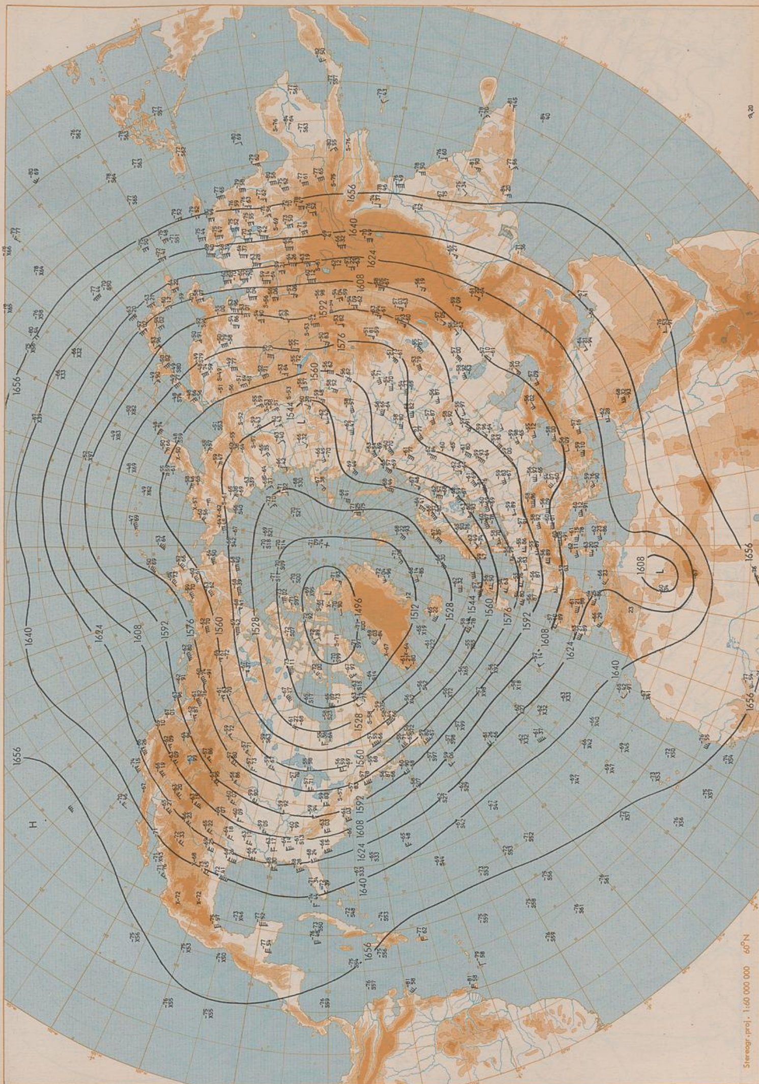
100 hPa 00 UTC
