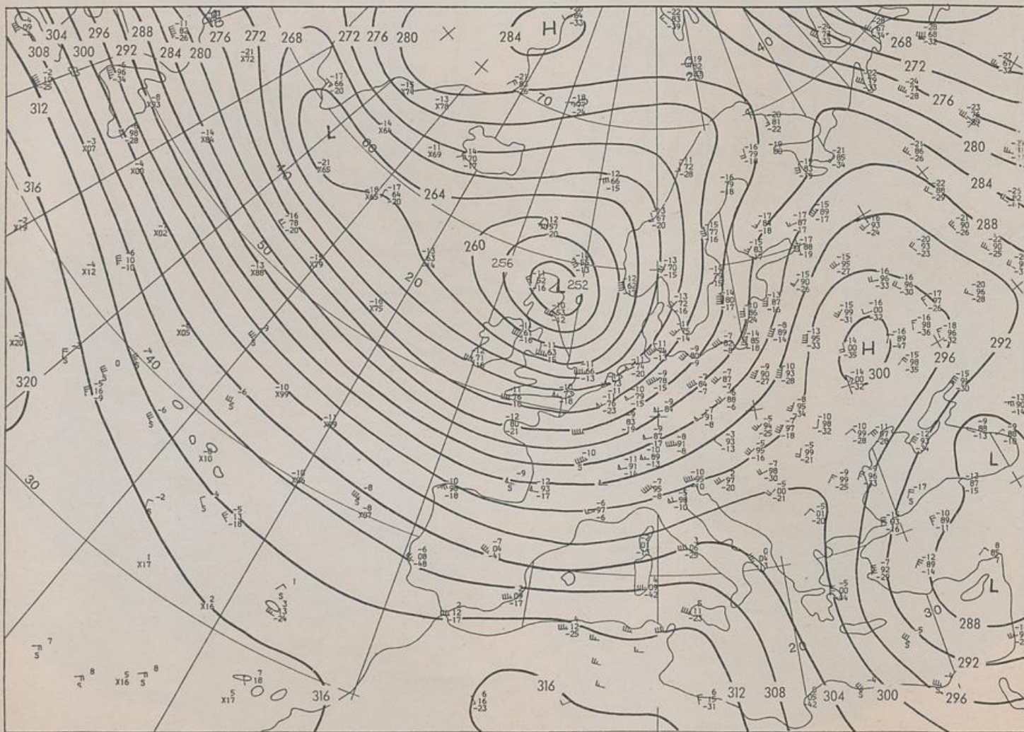
700 hPa 00 UTC
