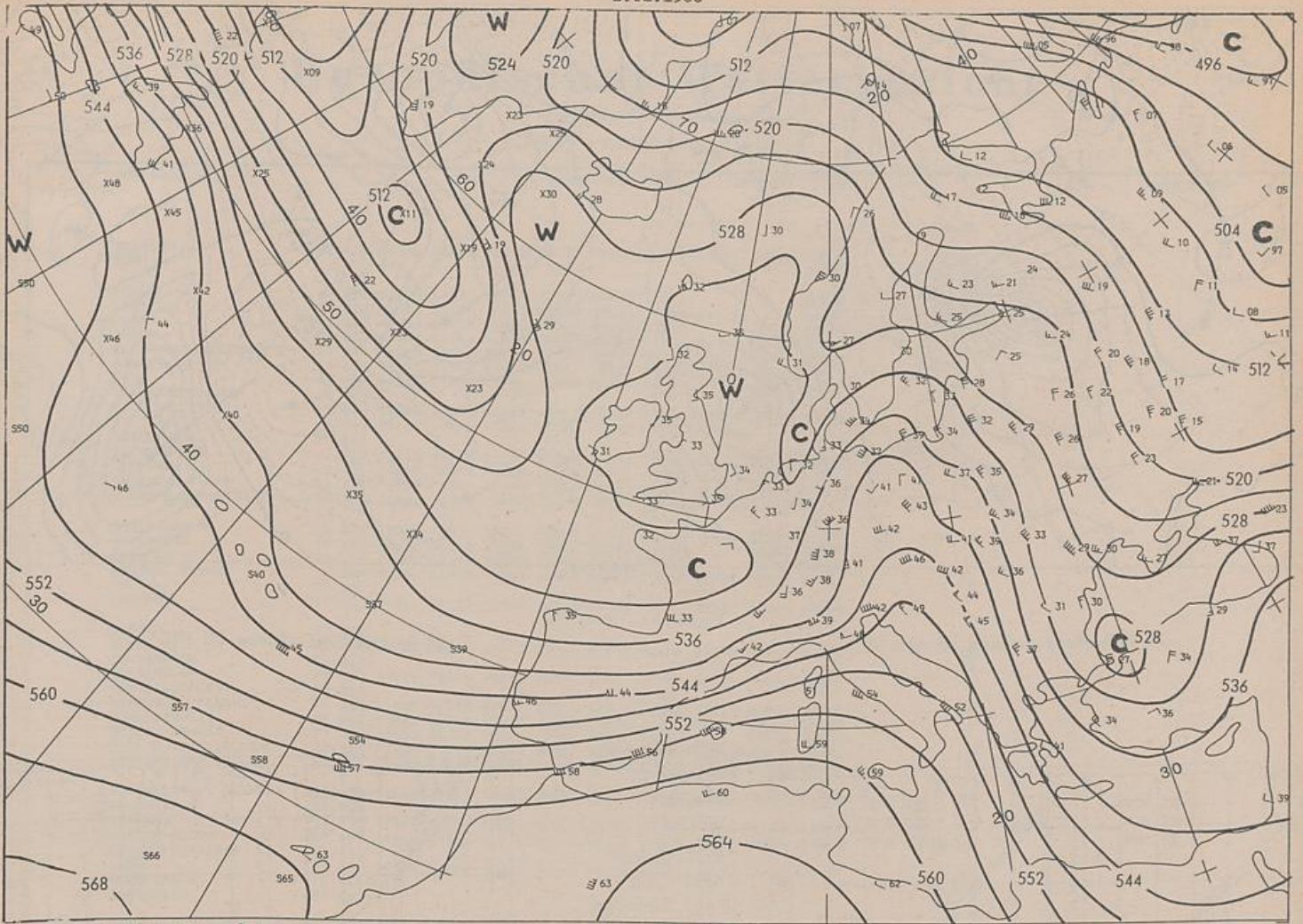
500/1000 hPa 00 UTC
