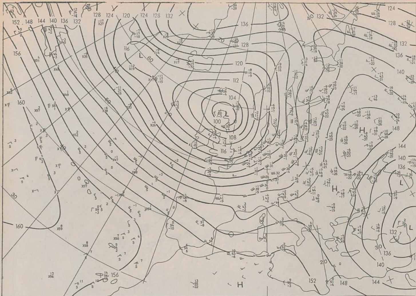
850 hPa 00 UTC
