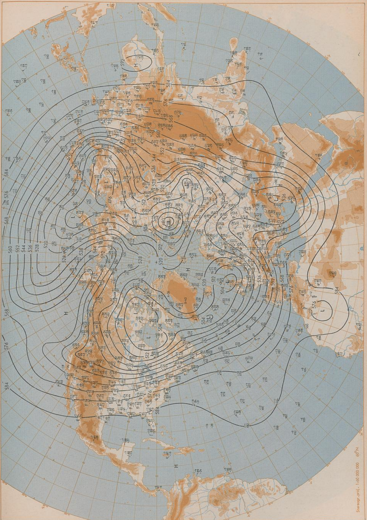
500 hPa 00 UTC
