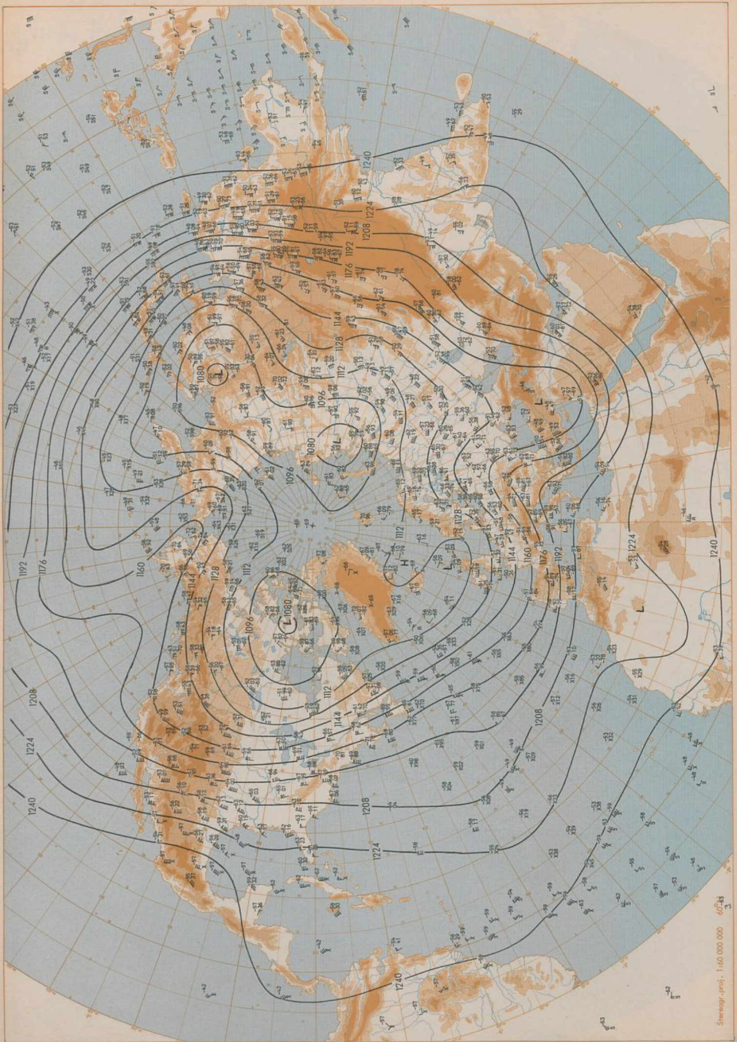
200 hPa 00 UTC
