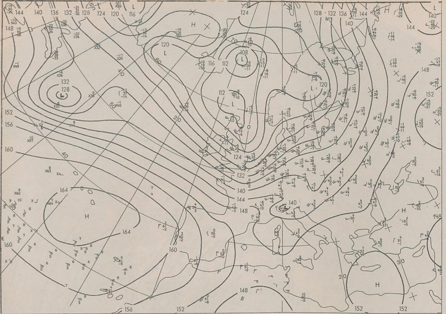
850 hPa 00 UTC
