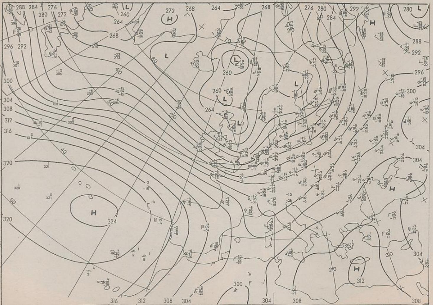
700 hPa 00 UTC
