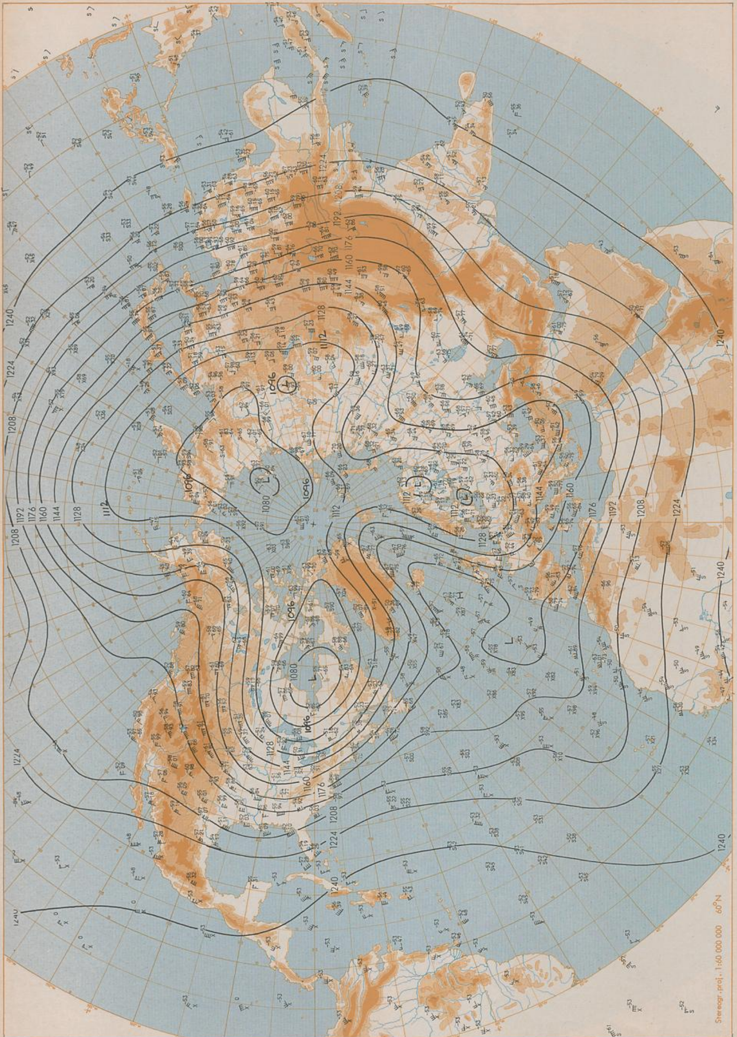
200 hPa 00 UTC
