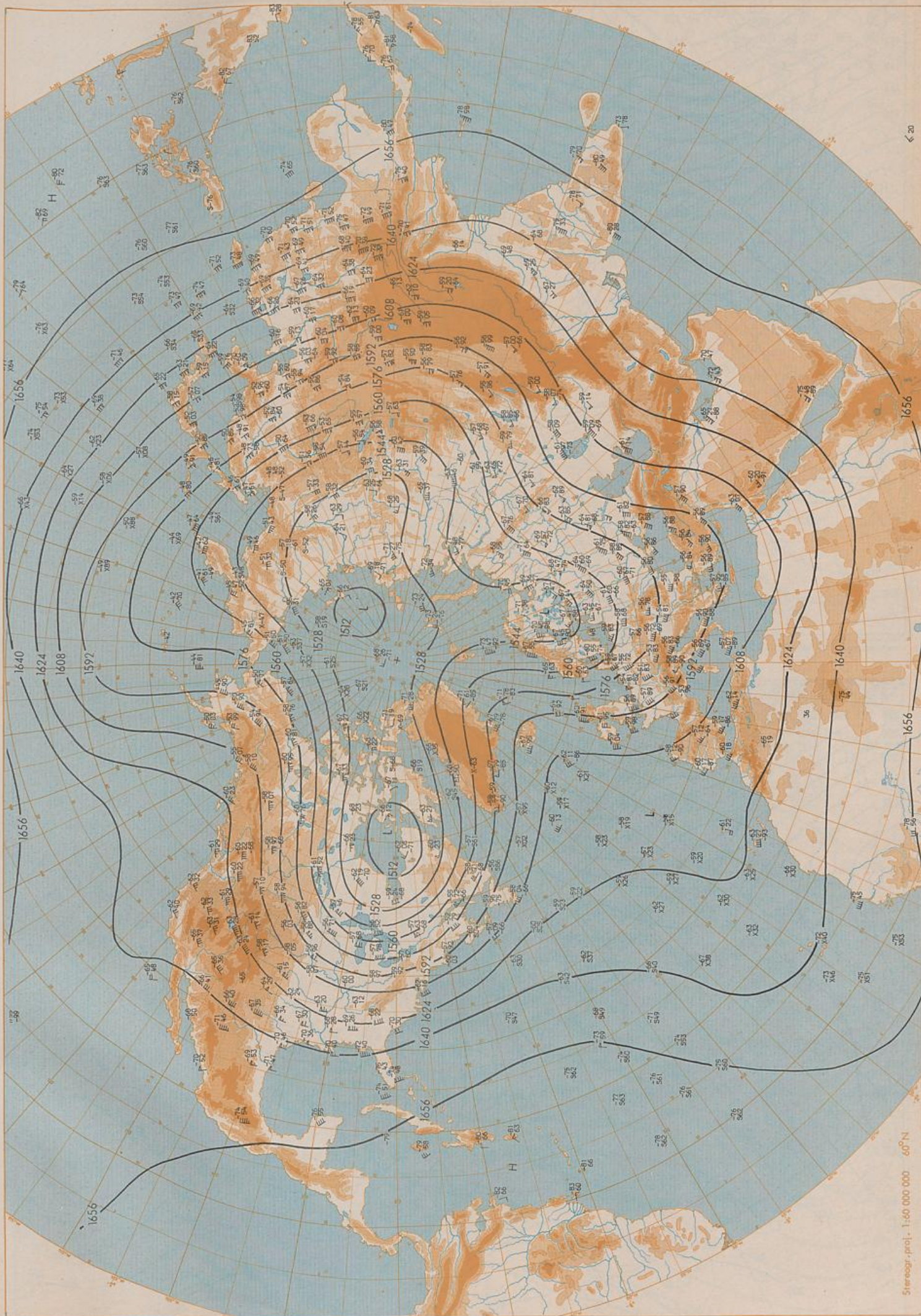
100 hPa 00 UTC
