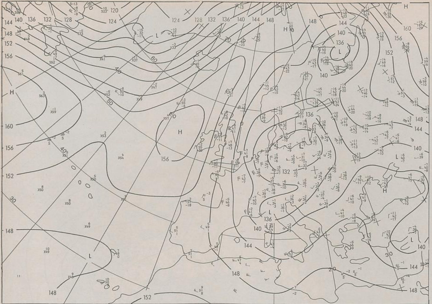
850 hPa 00 UTC
