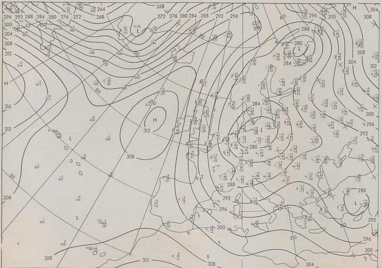
700 hPa 00 UTC
