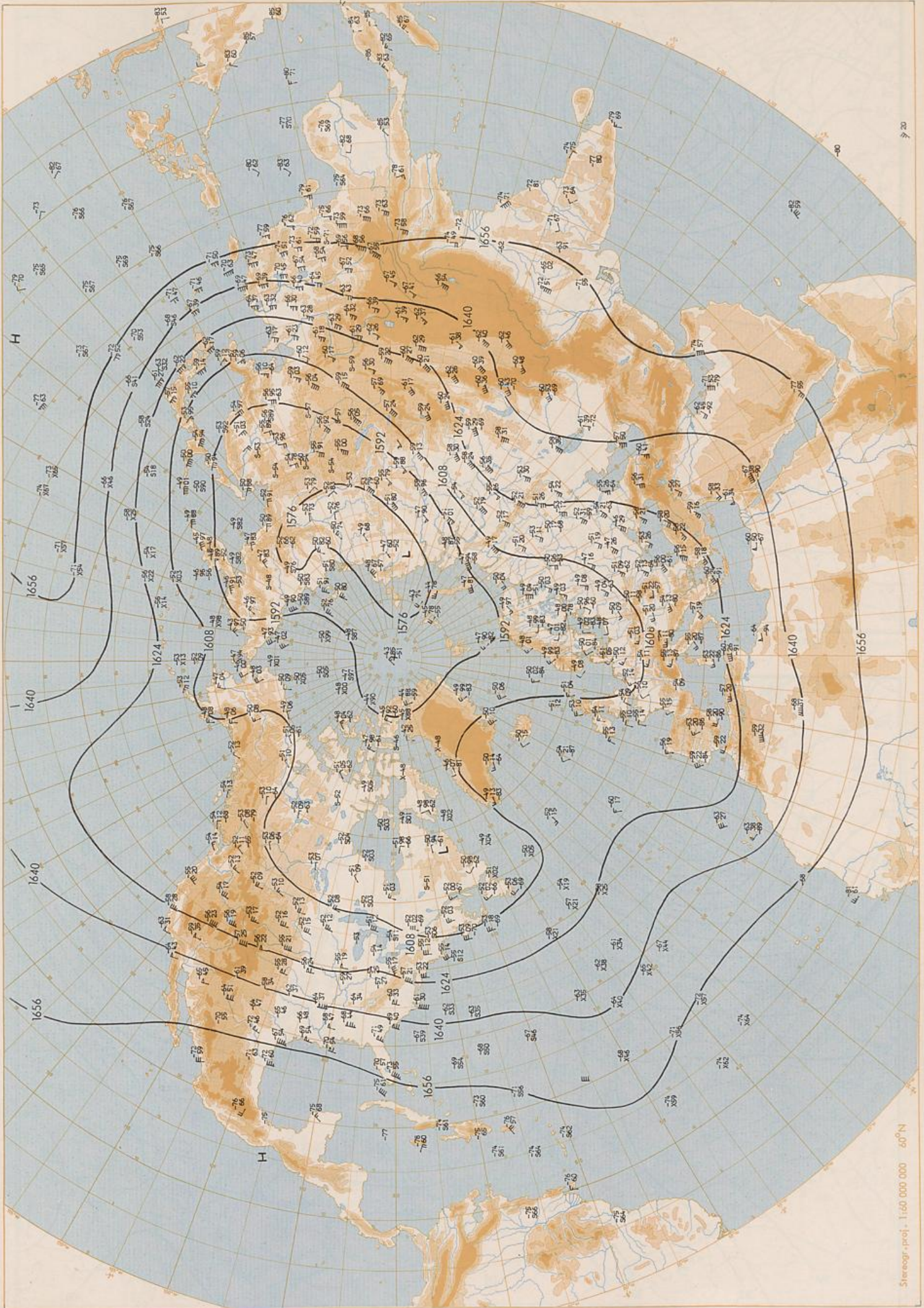
100 hPa 00 UTC
