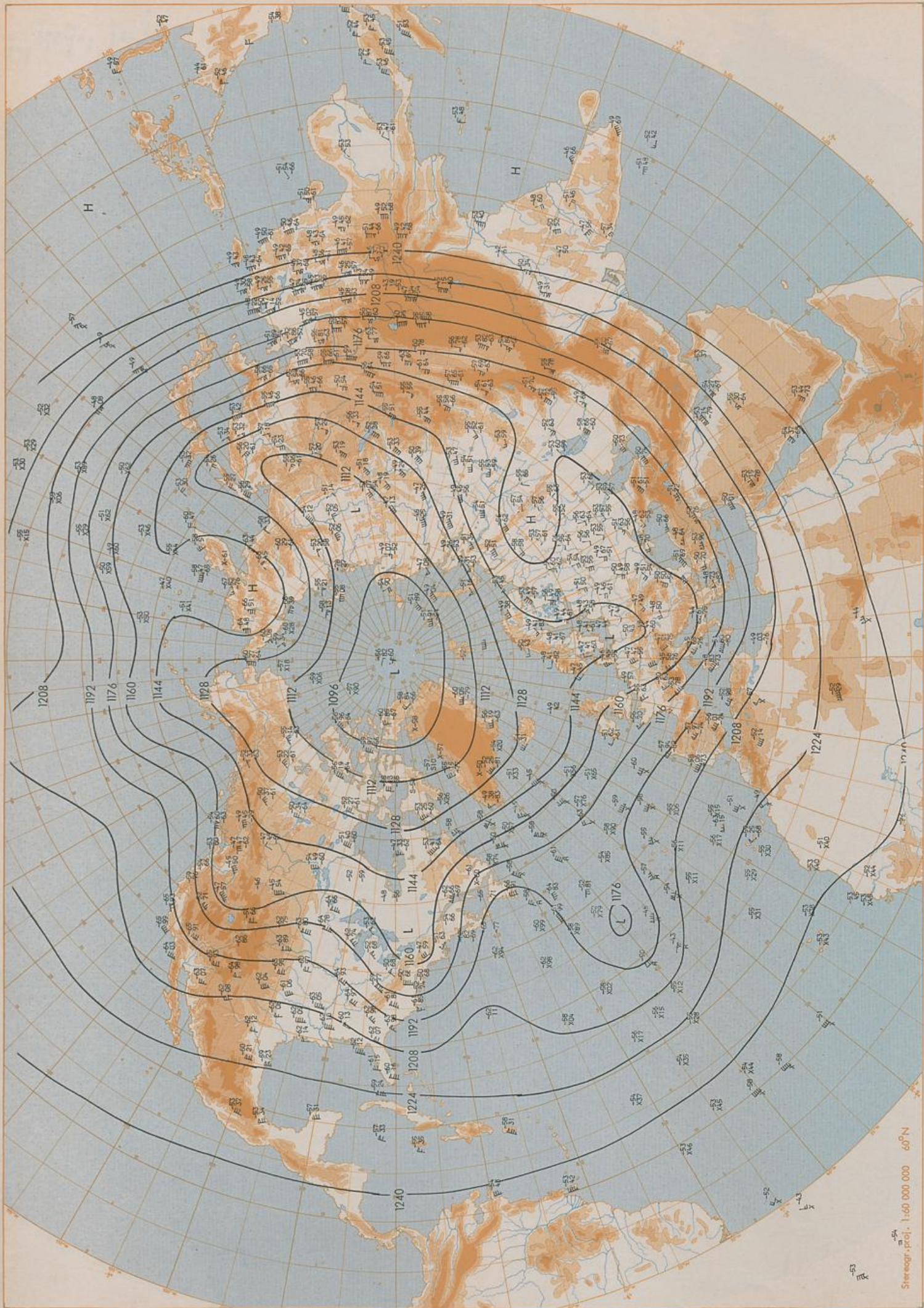
200 hPa 00 UTC
