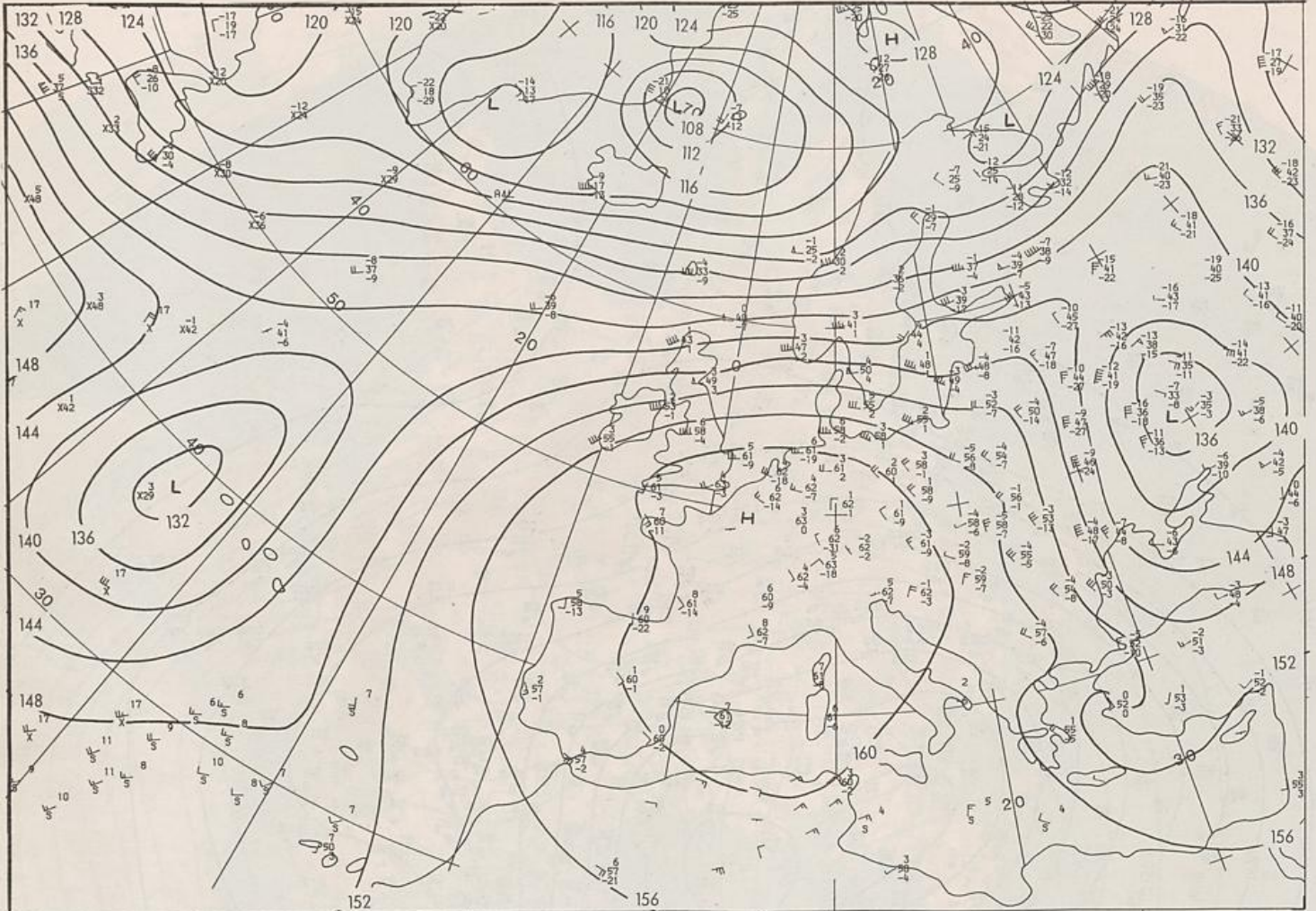
850 hPa 00 UTC
