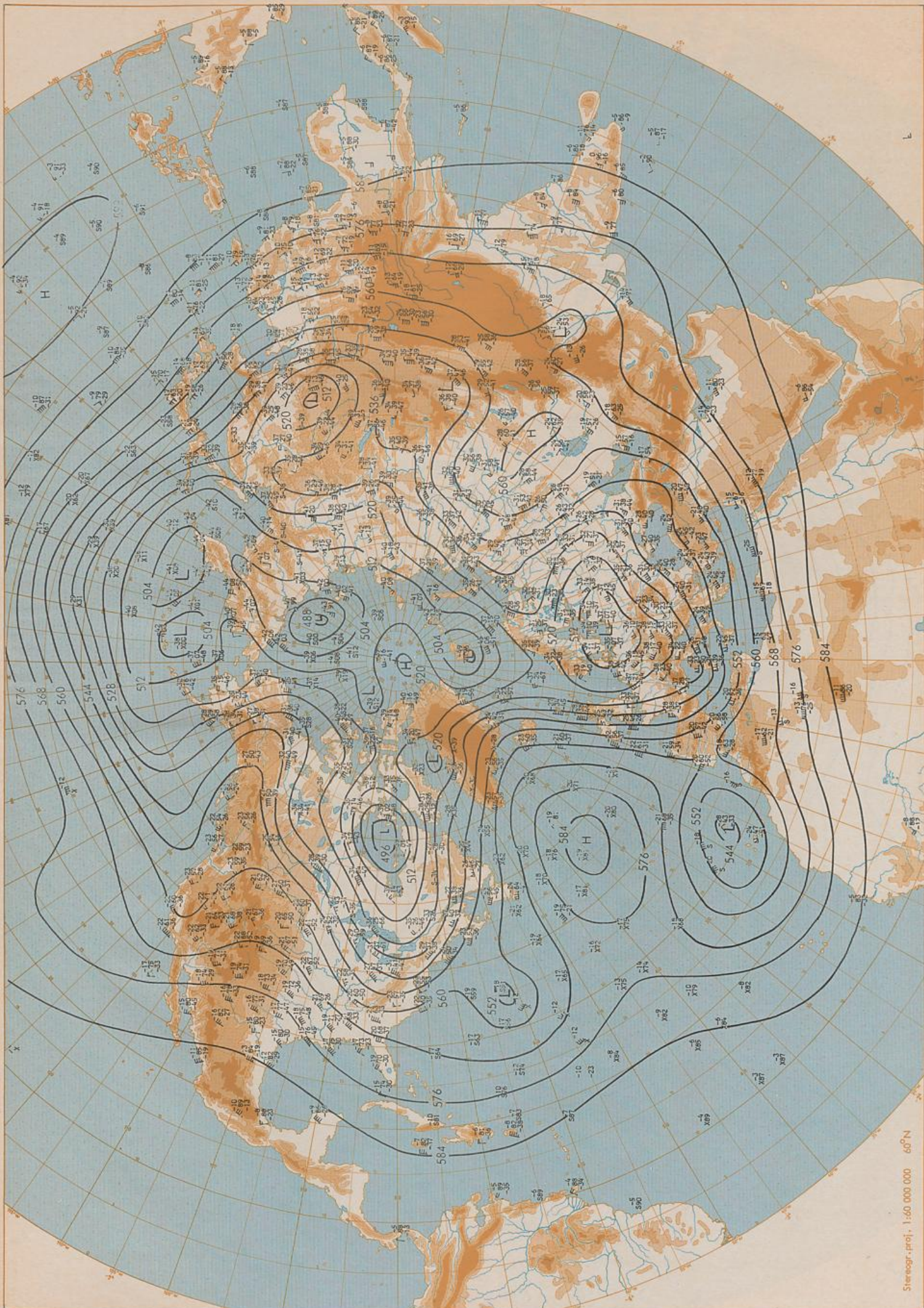
500 hPa 00 UTC
