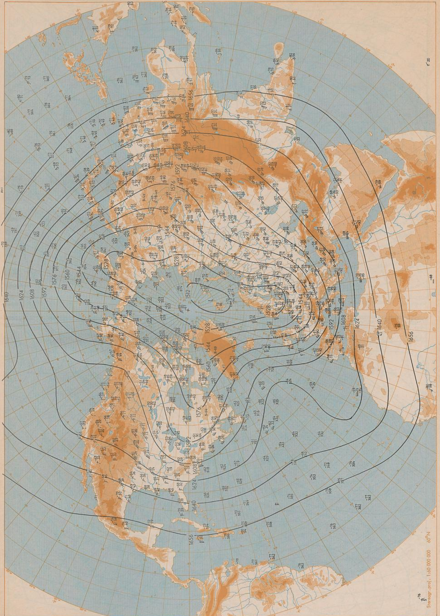
100 hPa 00 UTC
