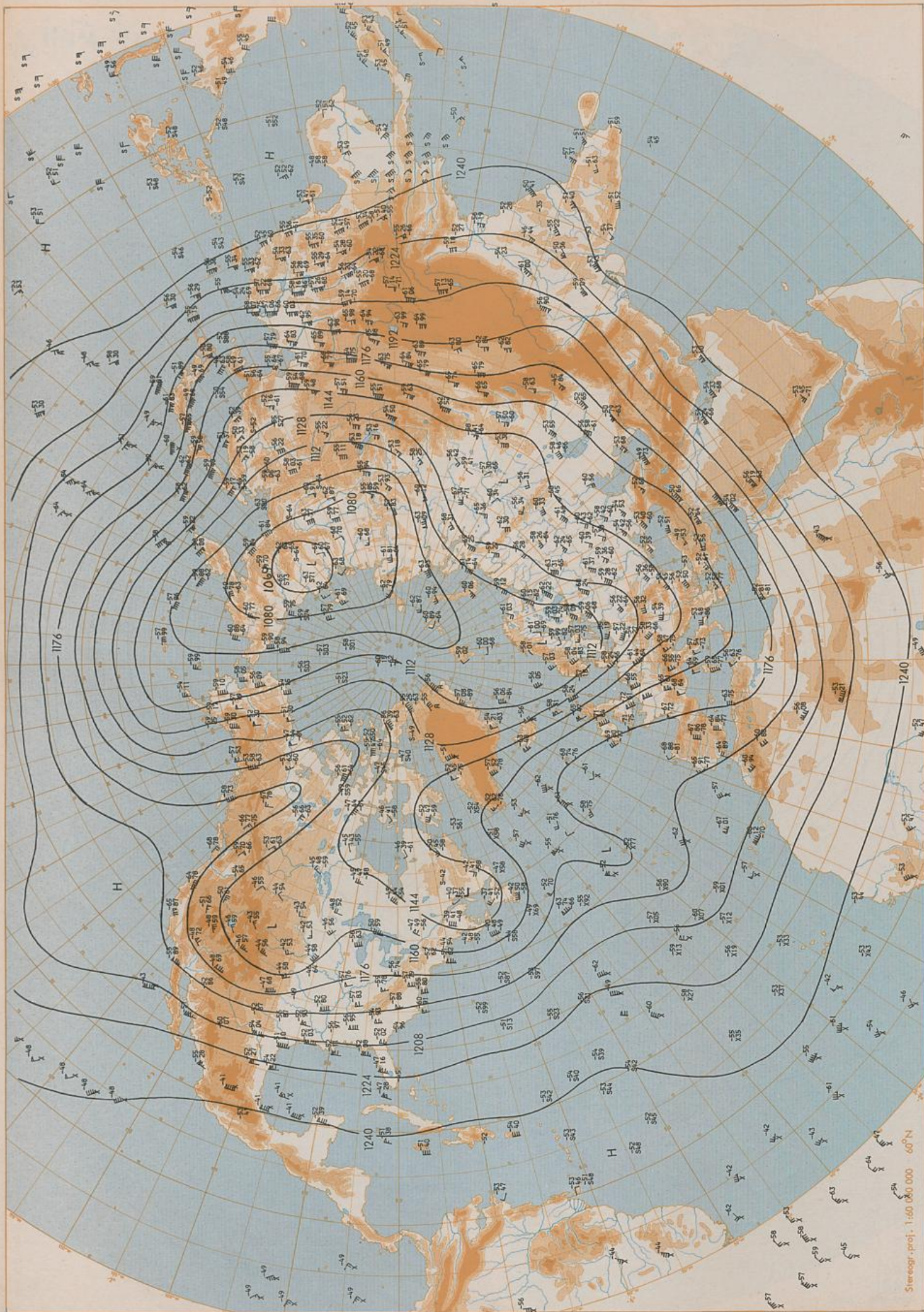
200 hPa 00 UTC
