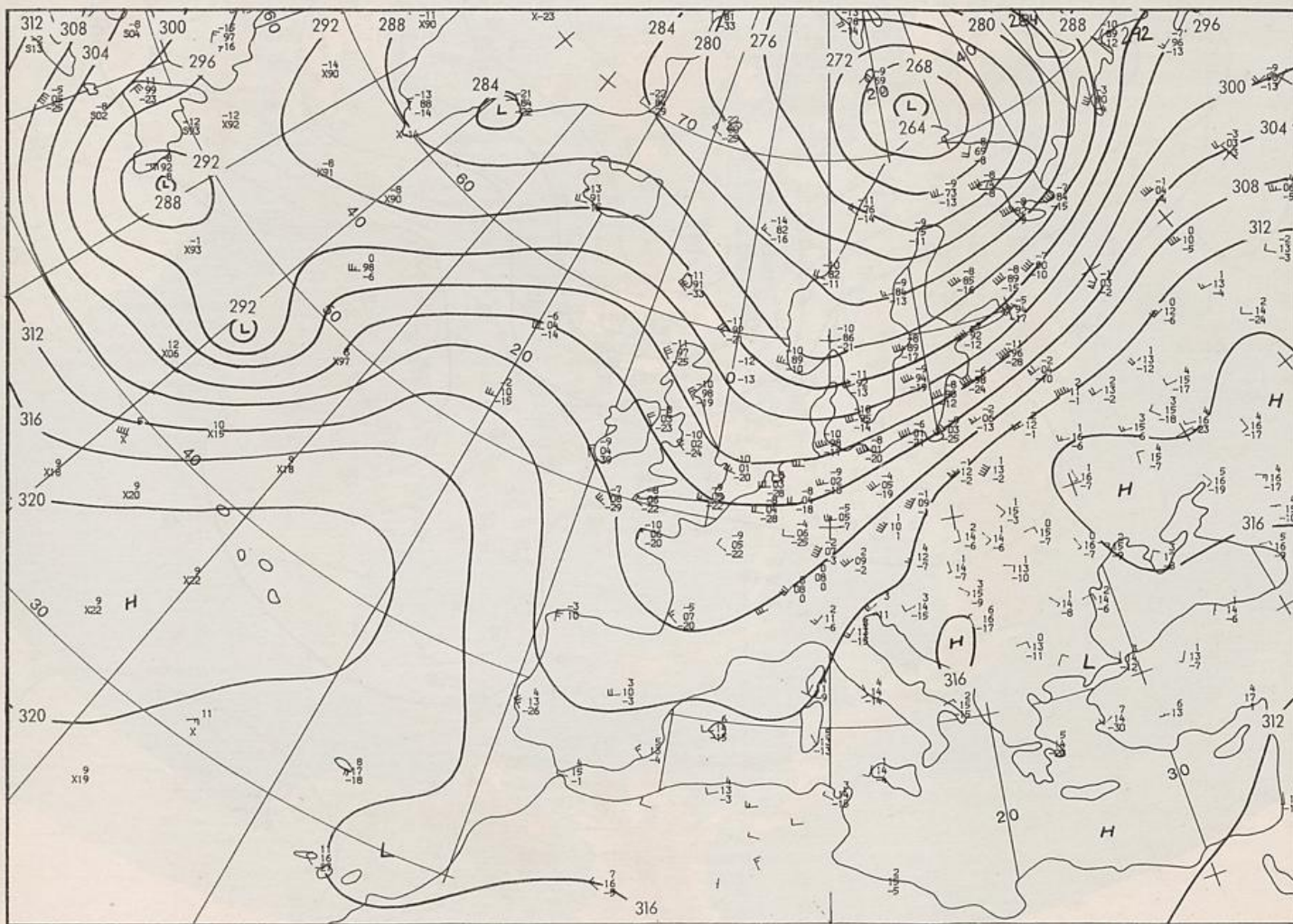
700 hPa 00 UTC
