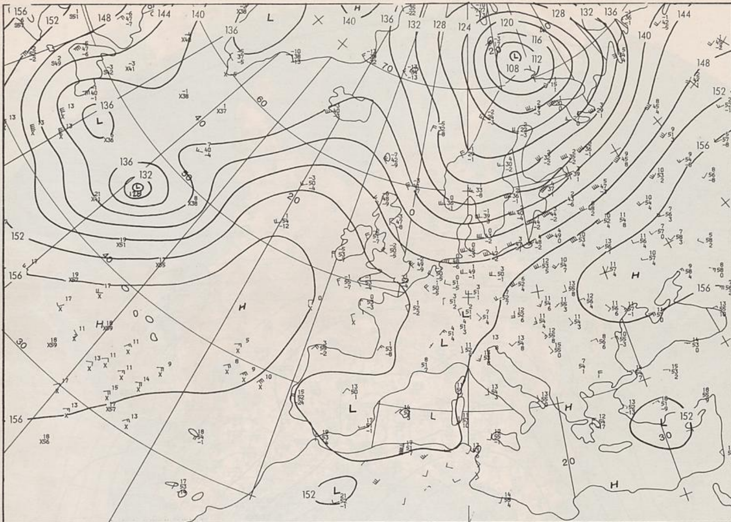
850 hPa 00 UTC
