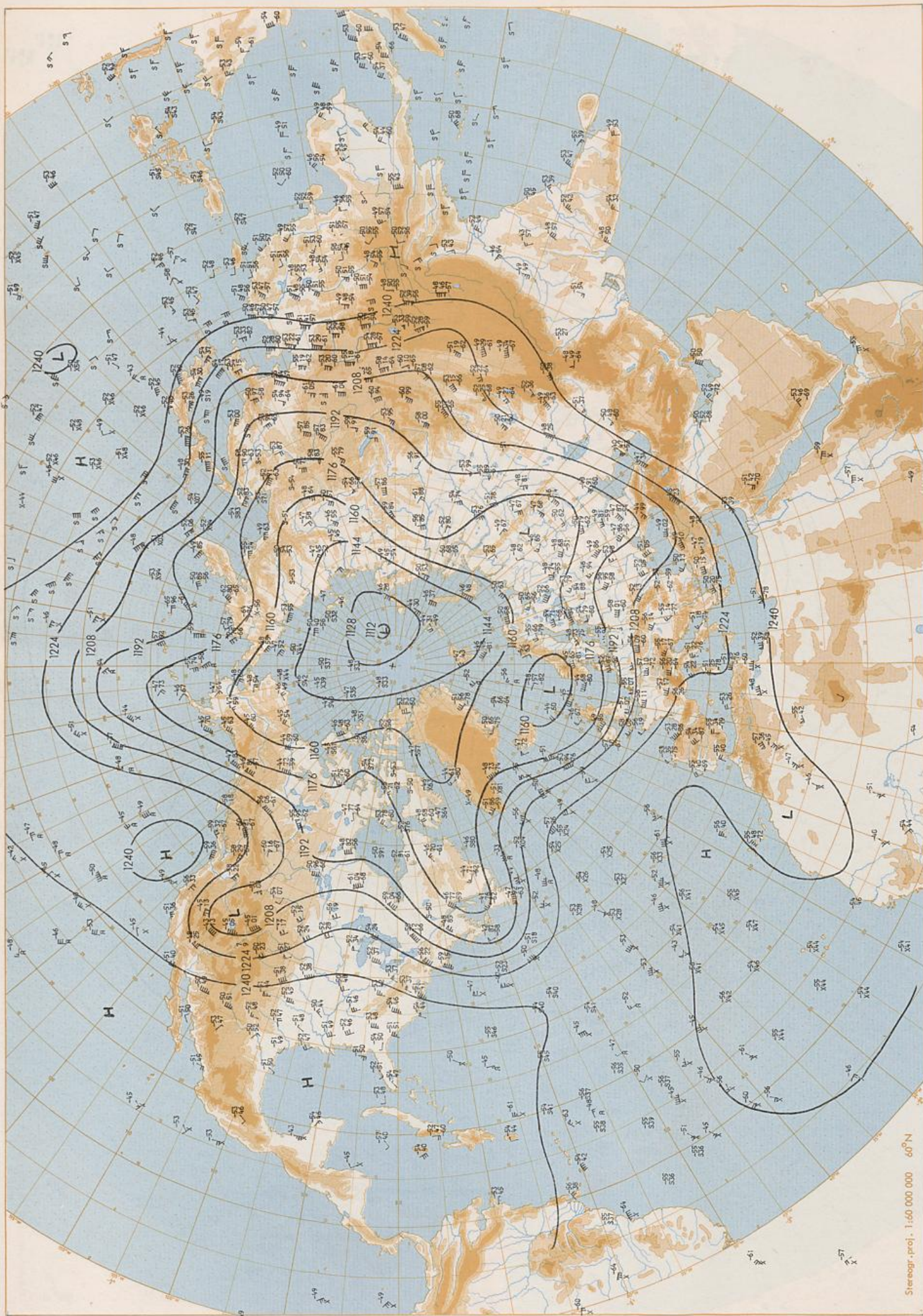
200 hPa 00 UTC
