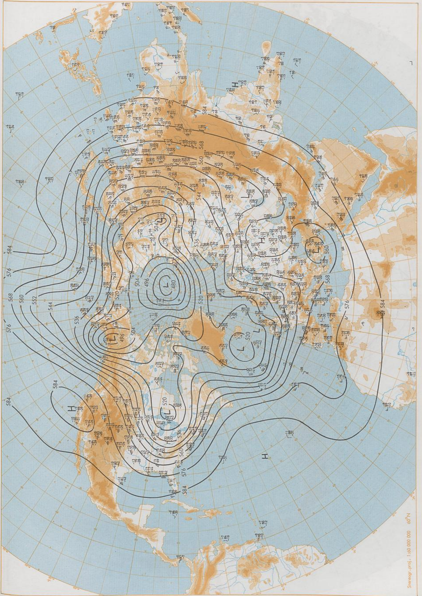
500 hPa 00 UTC
