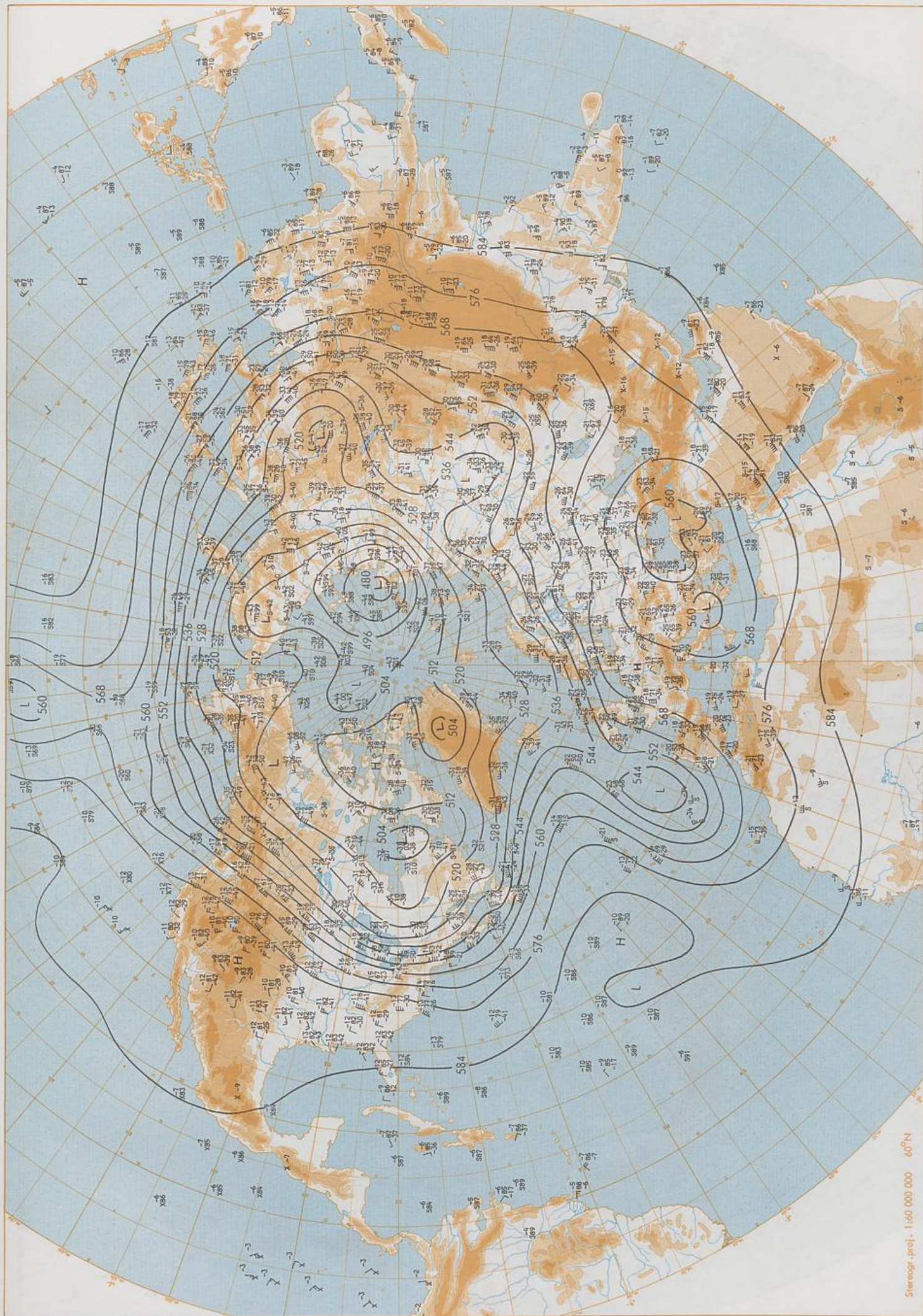
500 hPa 00 UTC
