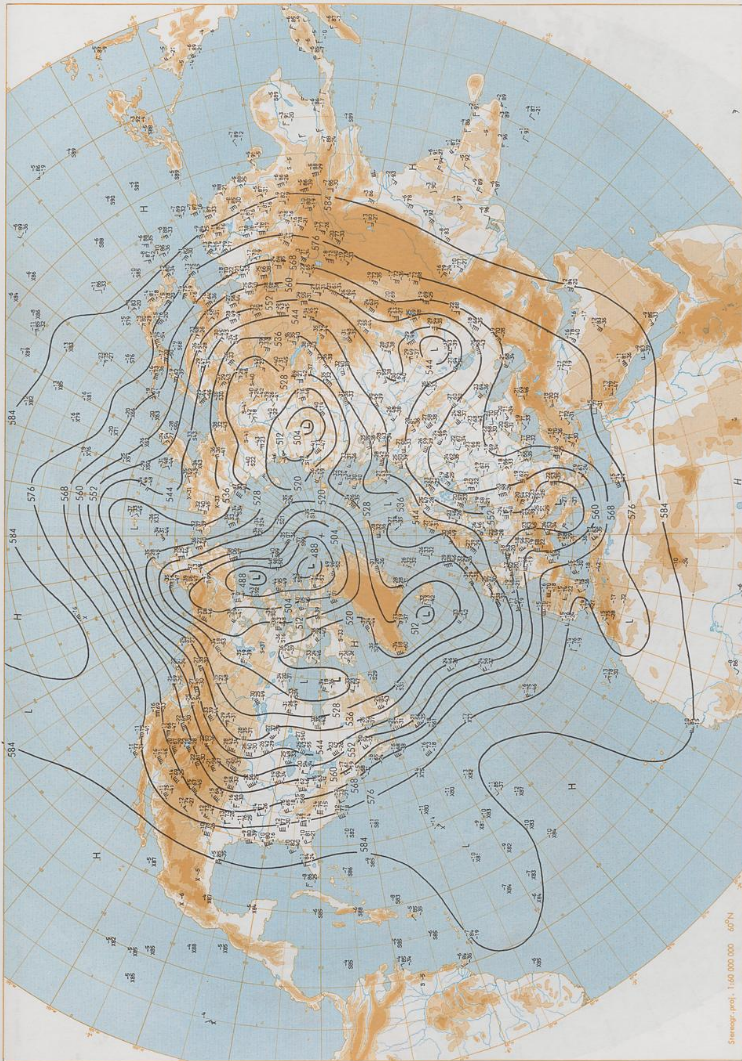
500 hPa 00 UTC
