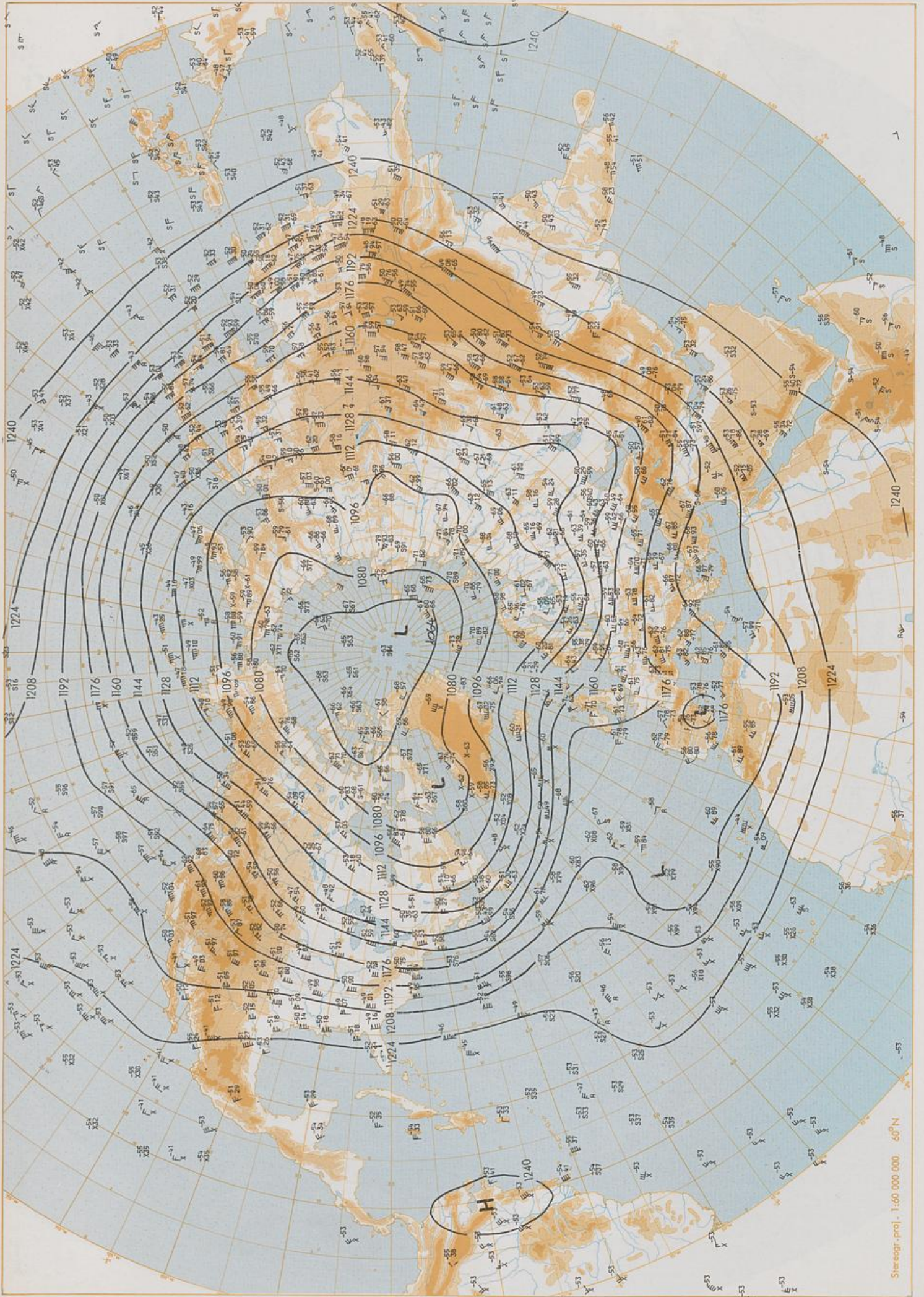
200 hPa 00 UTC
