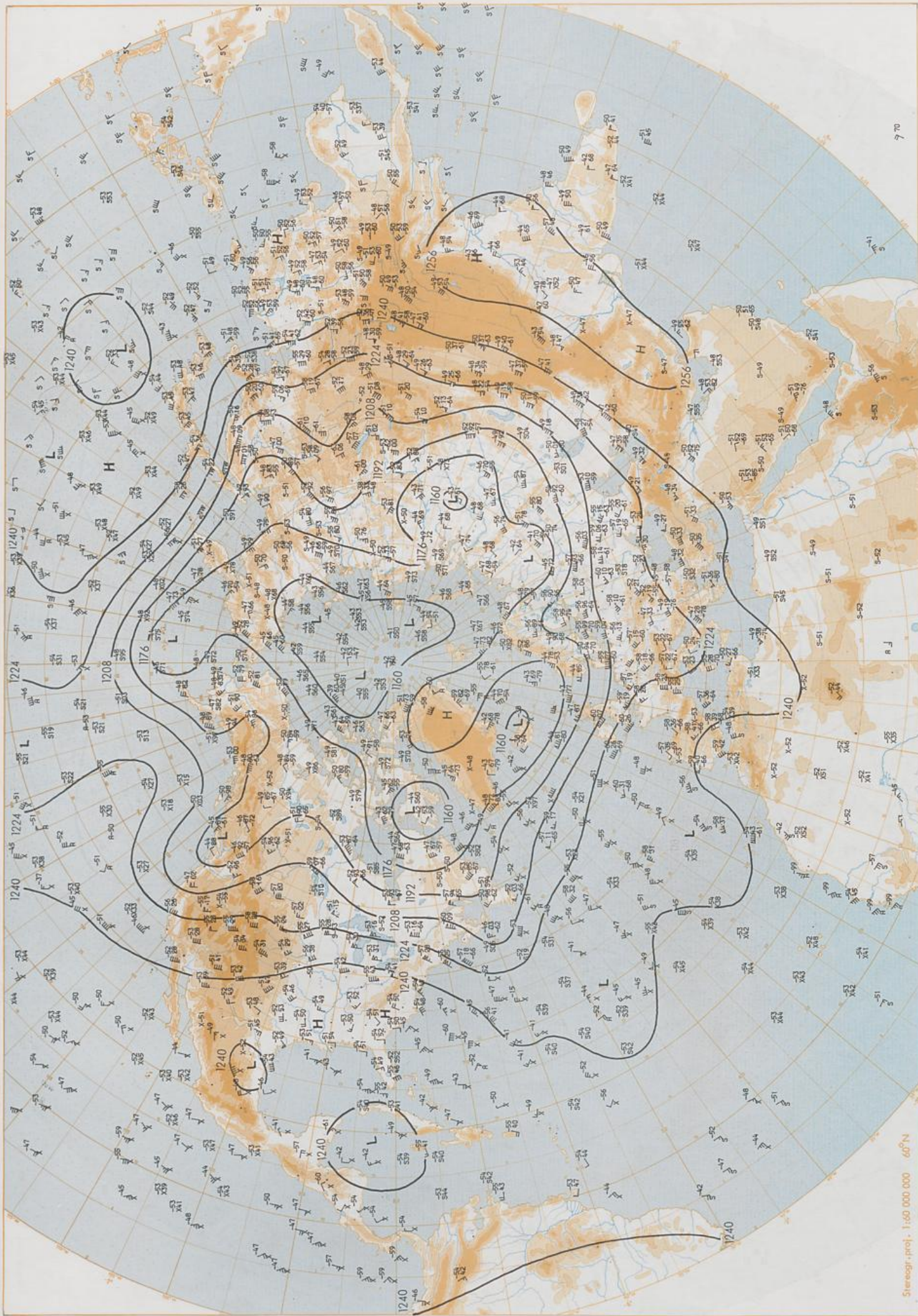
200 hPa 00 UTC
