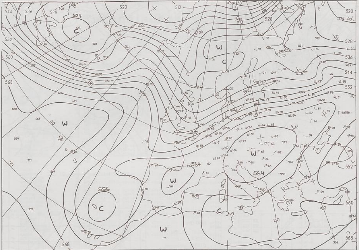
500/1000 hPa 00 UTC
