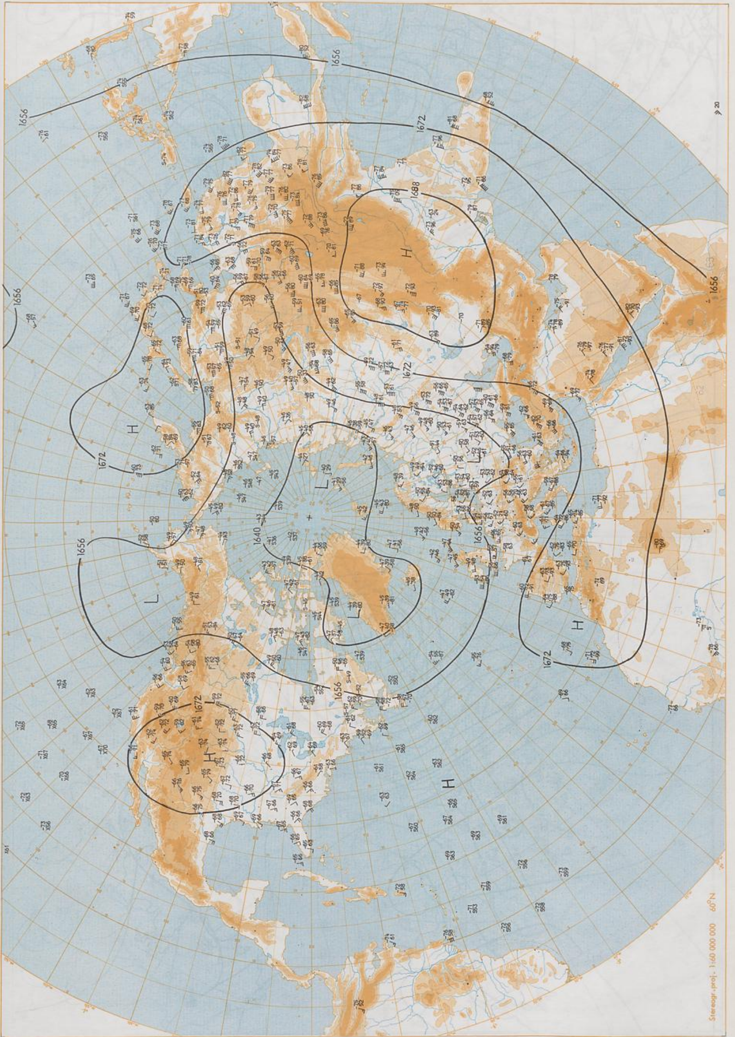
100 hPa 00 UTC
