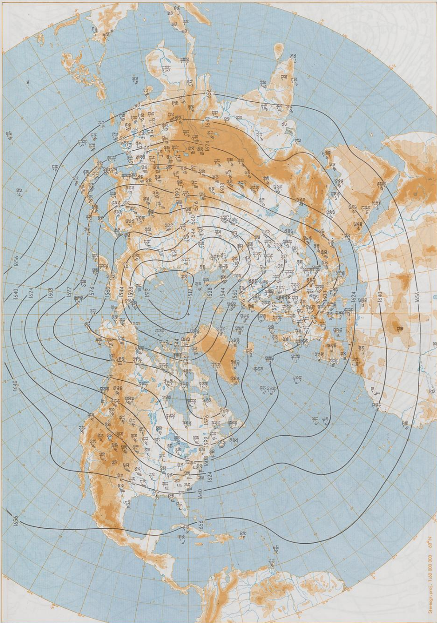
100 hPa 00 UTC
