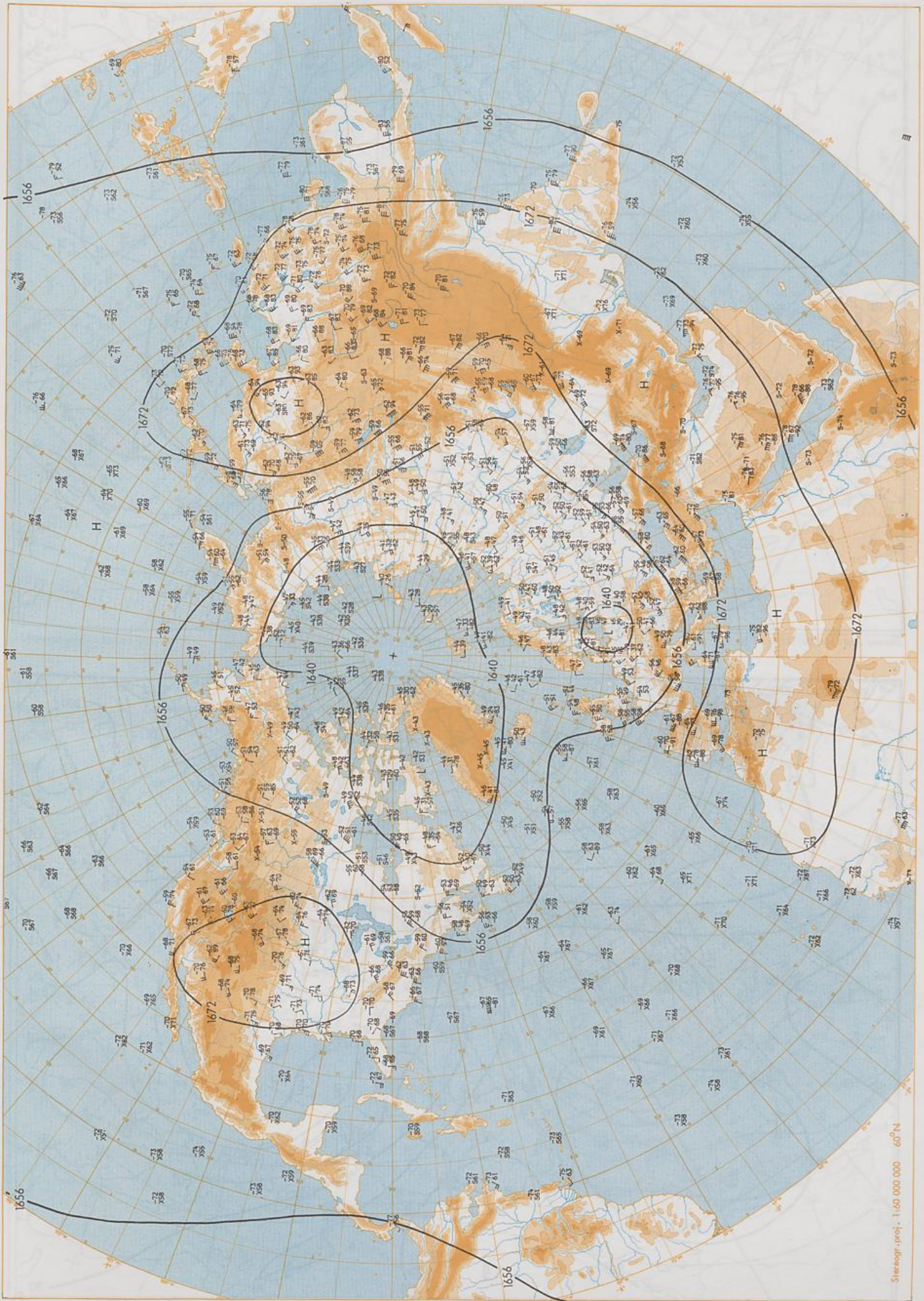
100 hPa 00 UTC
