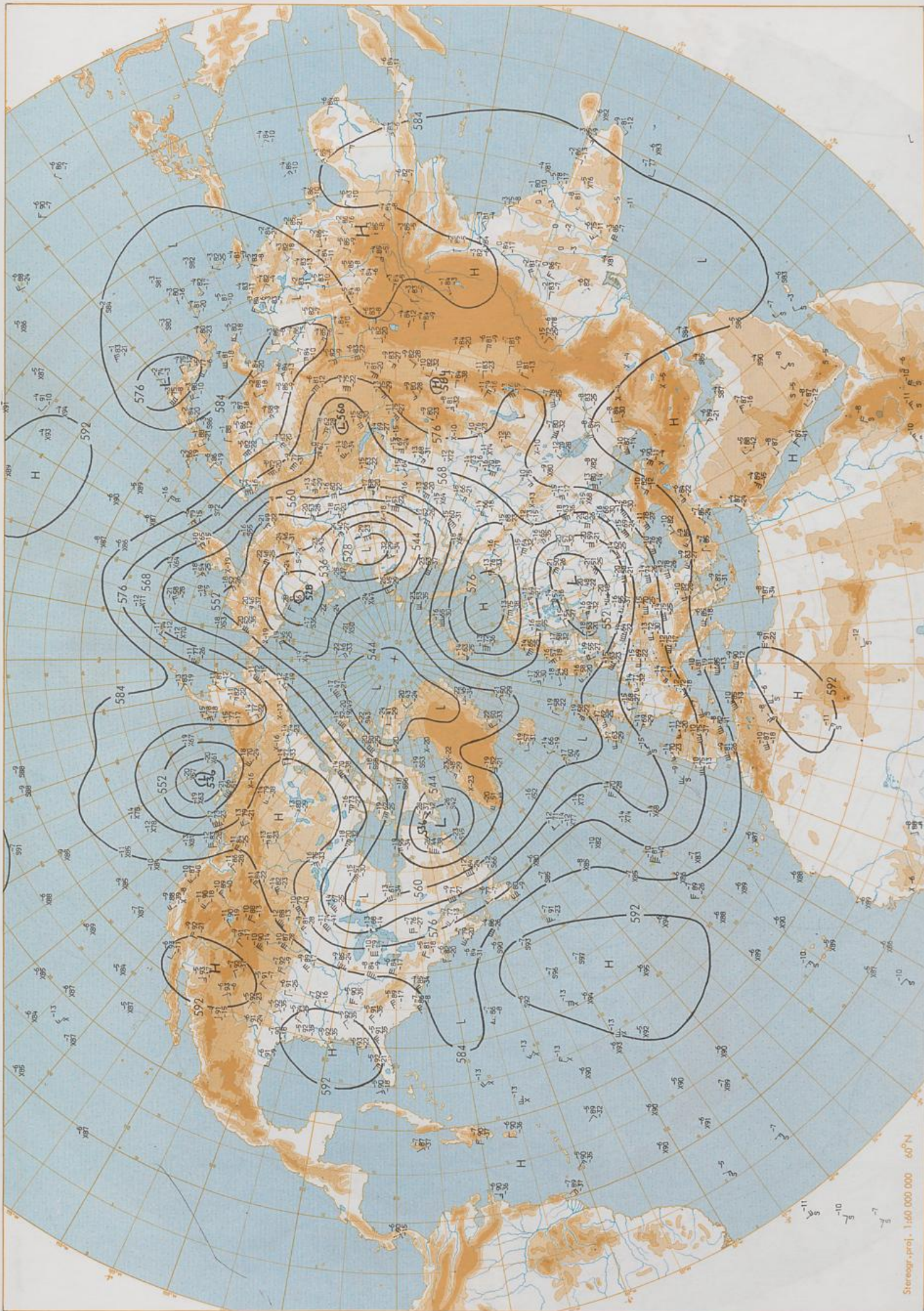
500 hPa 00 UTC
