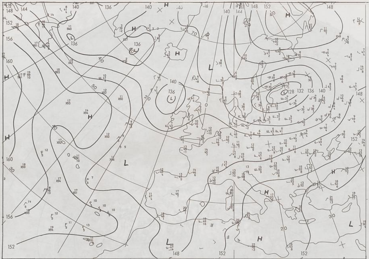
850 hPa 00 UTC
