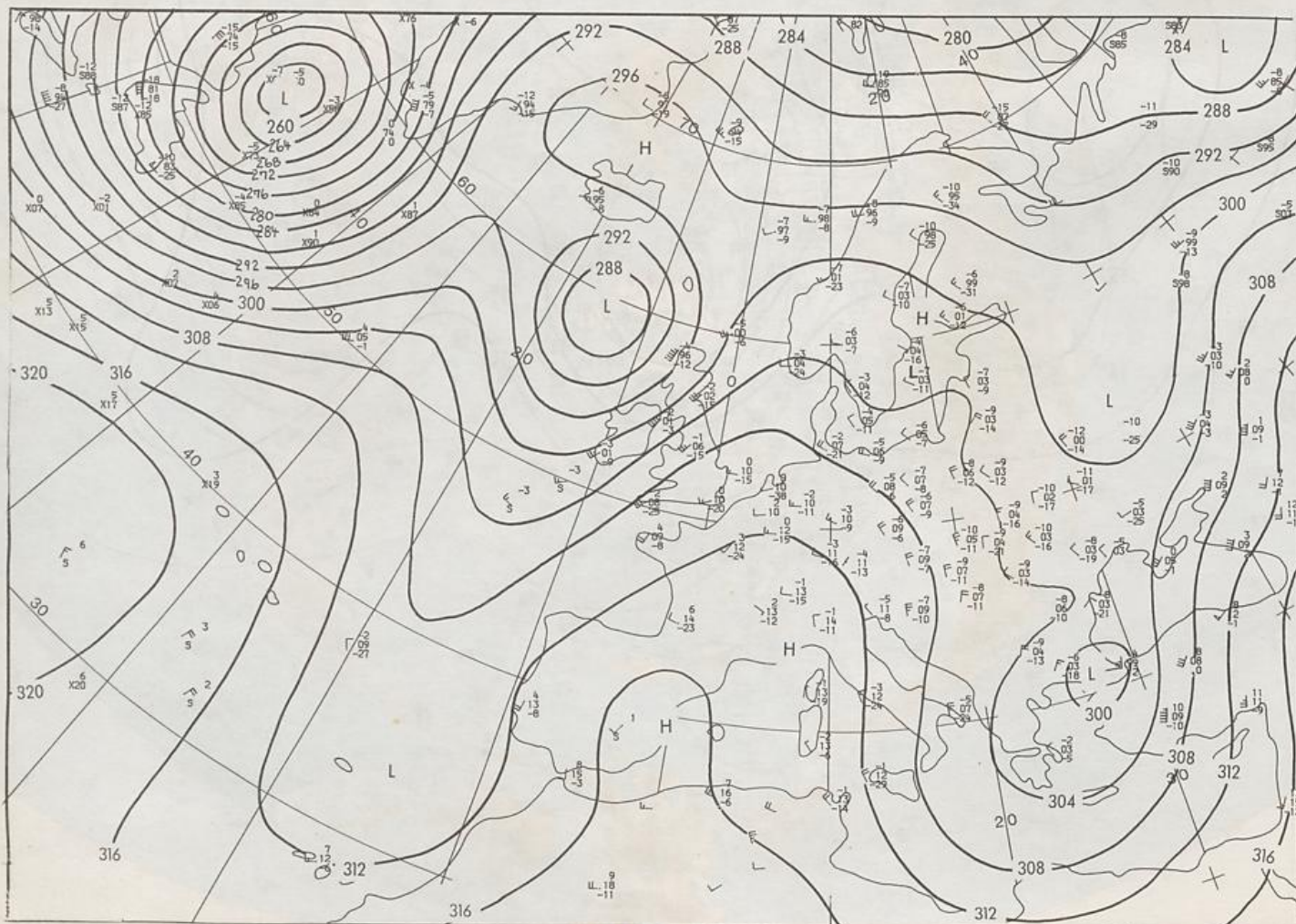
700 hPa 00 UTC
