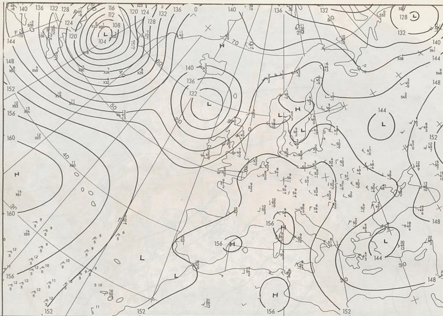
850 hPa 00 UTC
