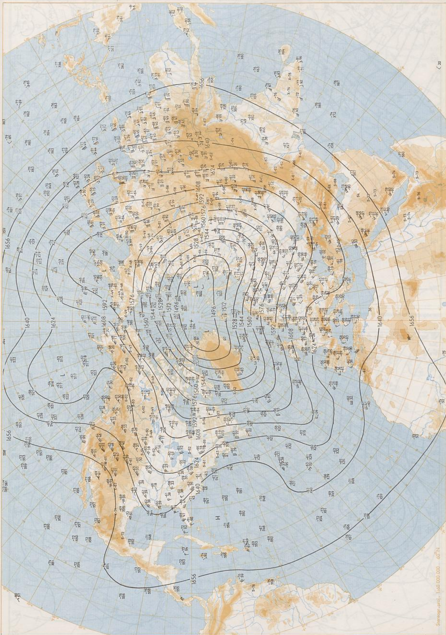
100 hPa 00 UTC
