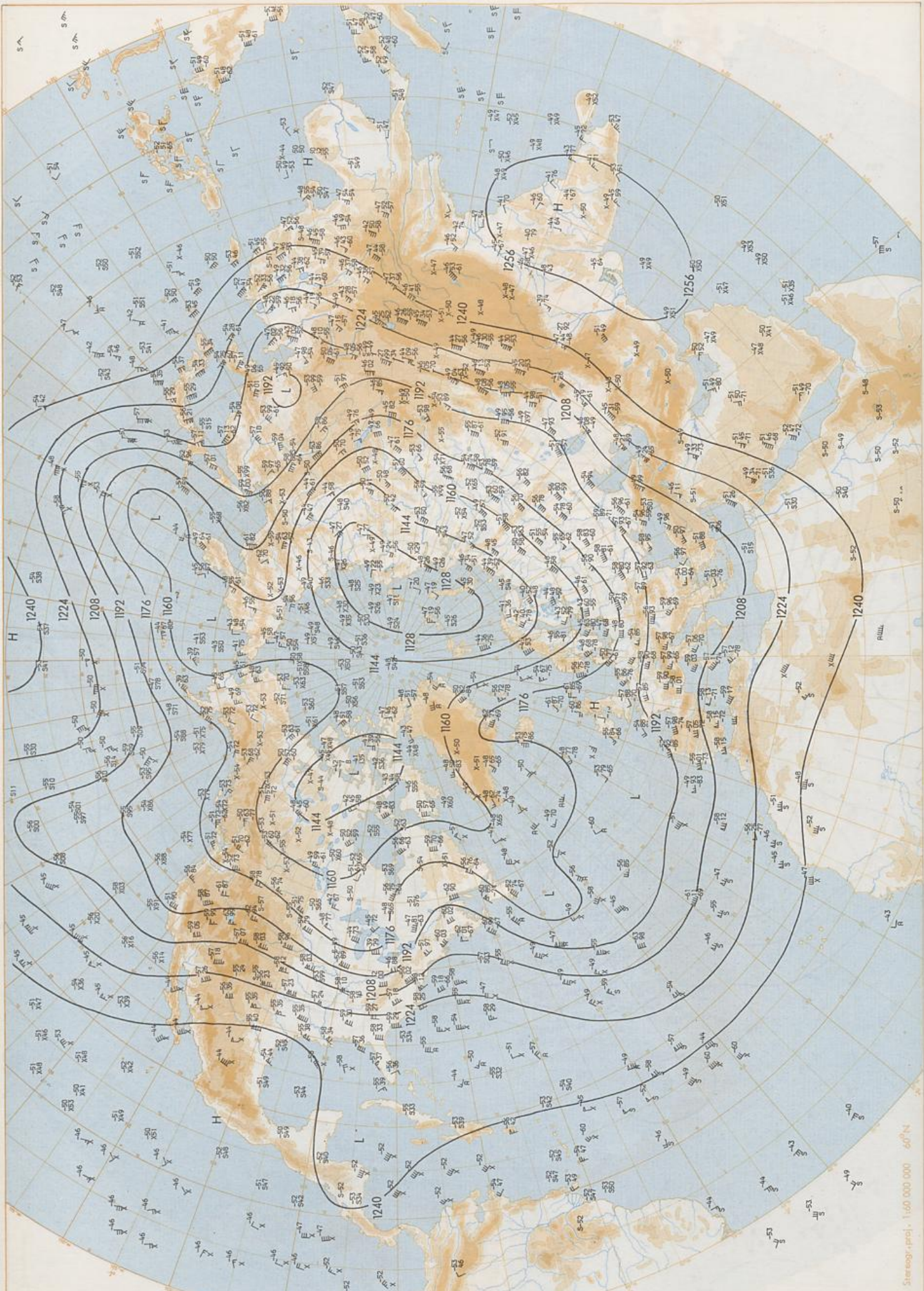
200 hPa 00 UTC
