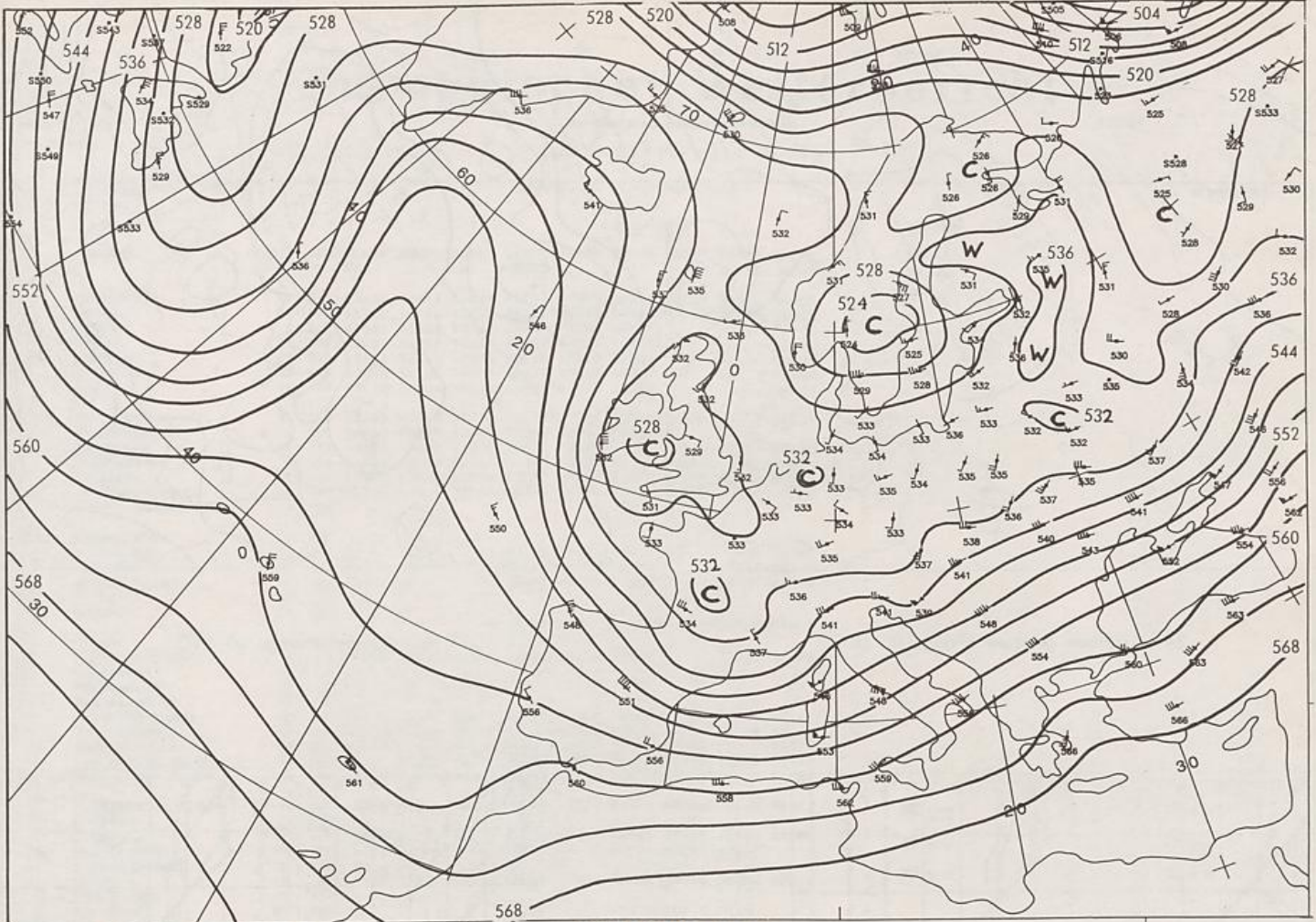
500/1000 hPa 00 UTC
