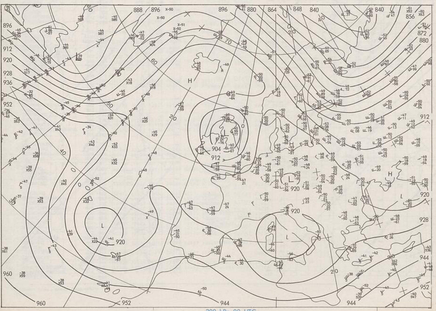
300 hPa 00 UTC
