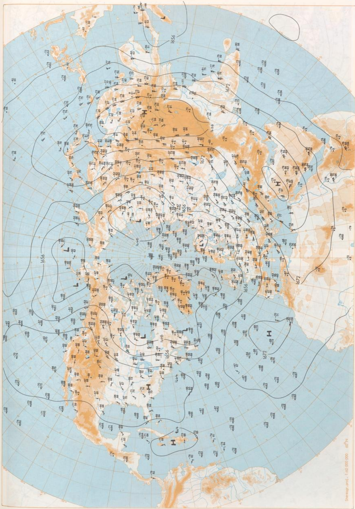
100 hPa 12 UTC
