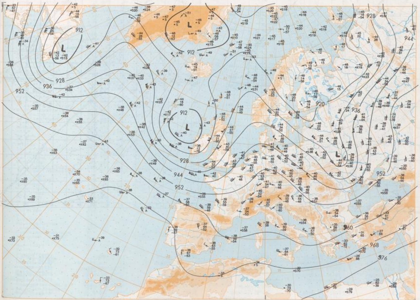
300 hPa 12 UTC
