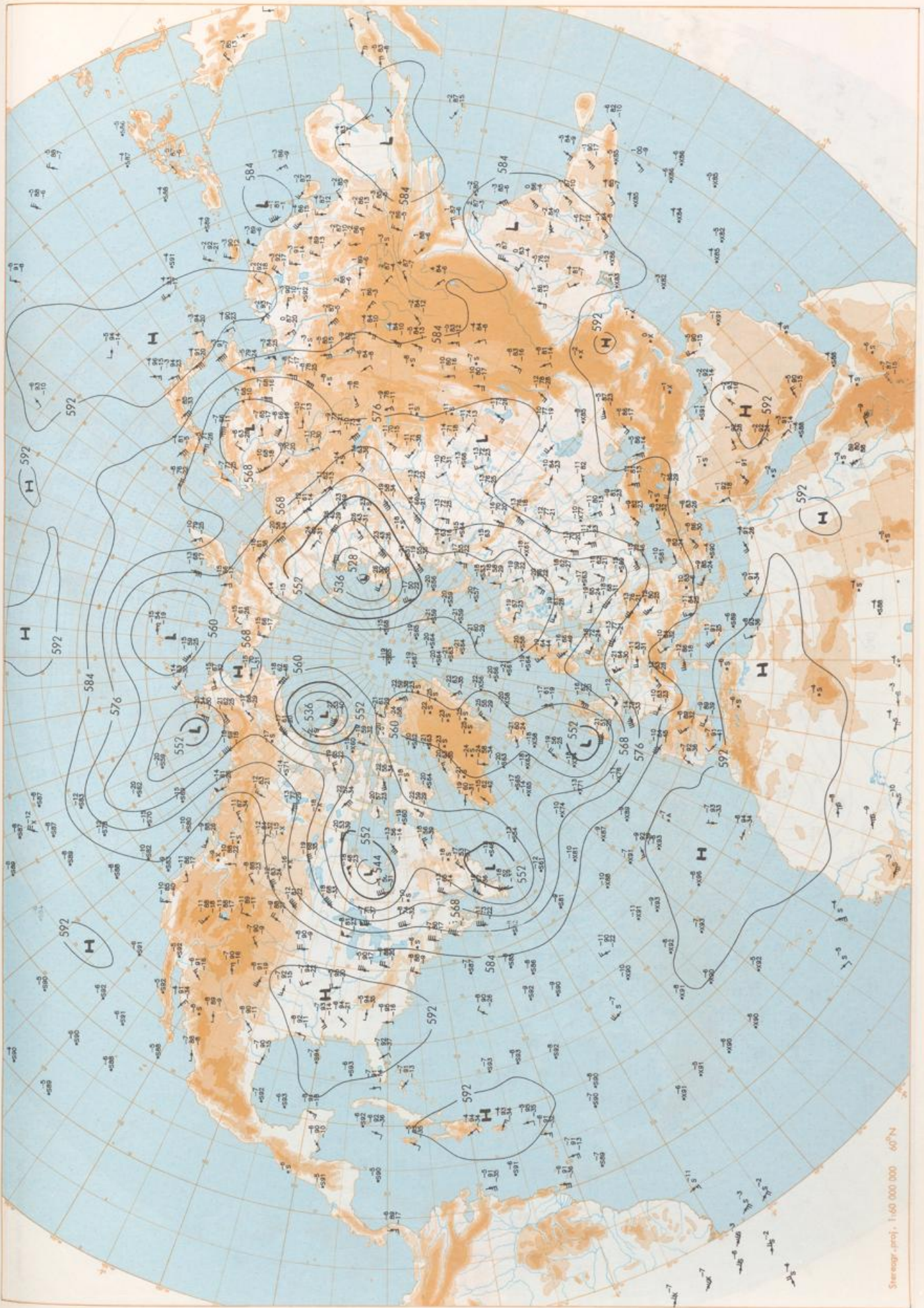
500 hPa 12 UTC
