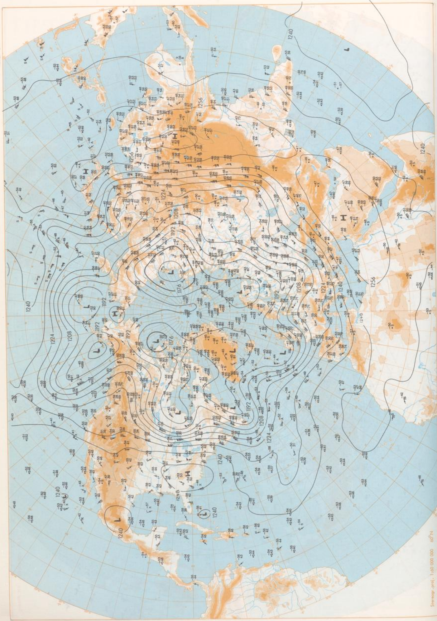
200 hPa 12 UTC
