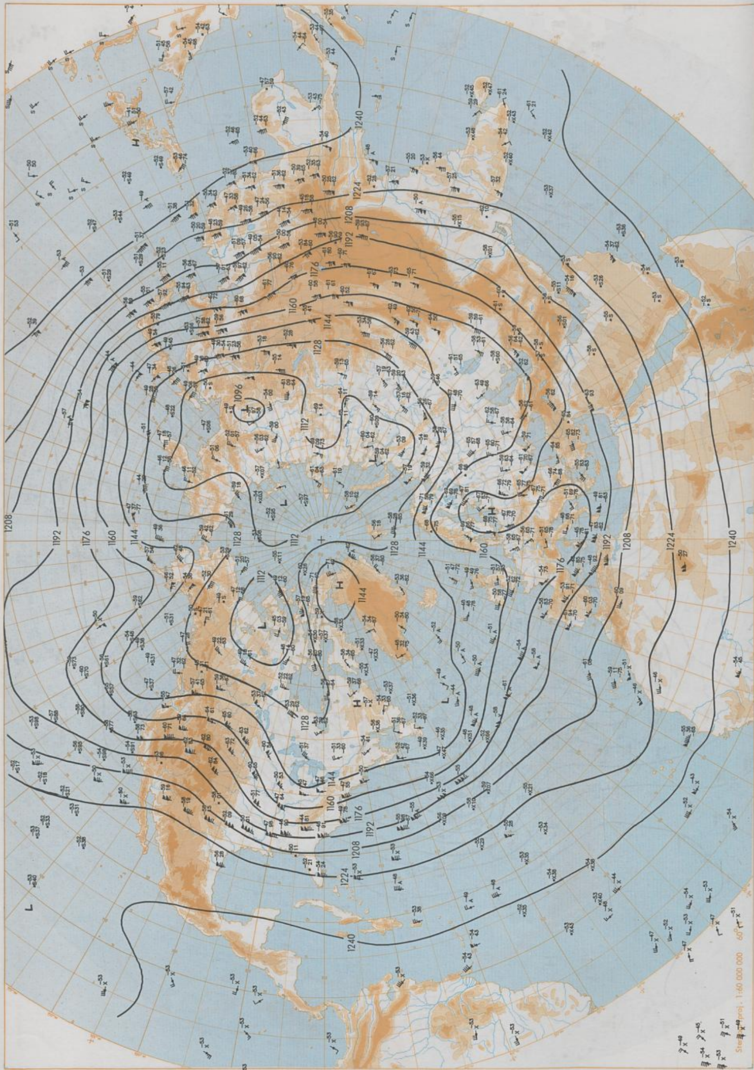
200 hPa 00 UTC
