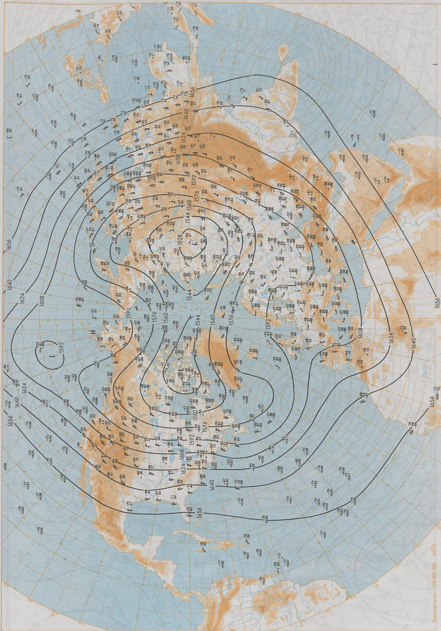
100 hPa 00 UTC
