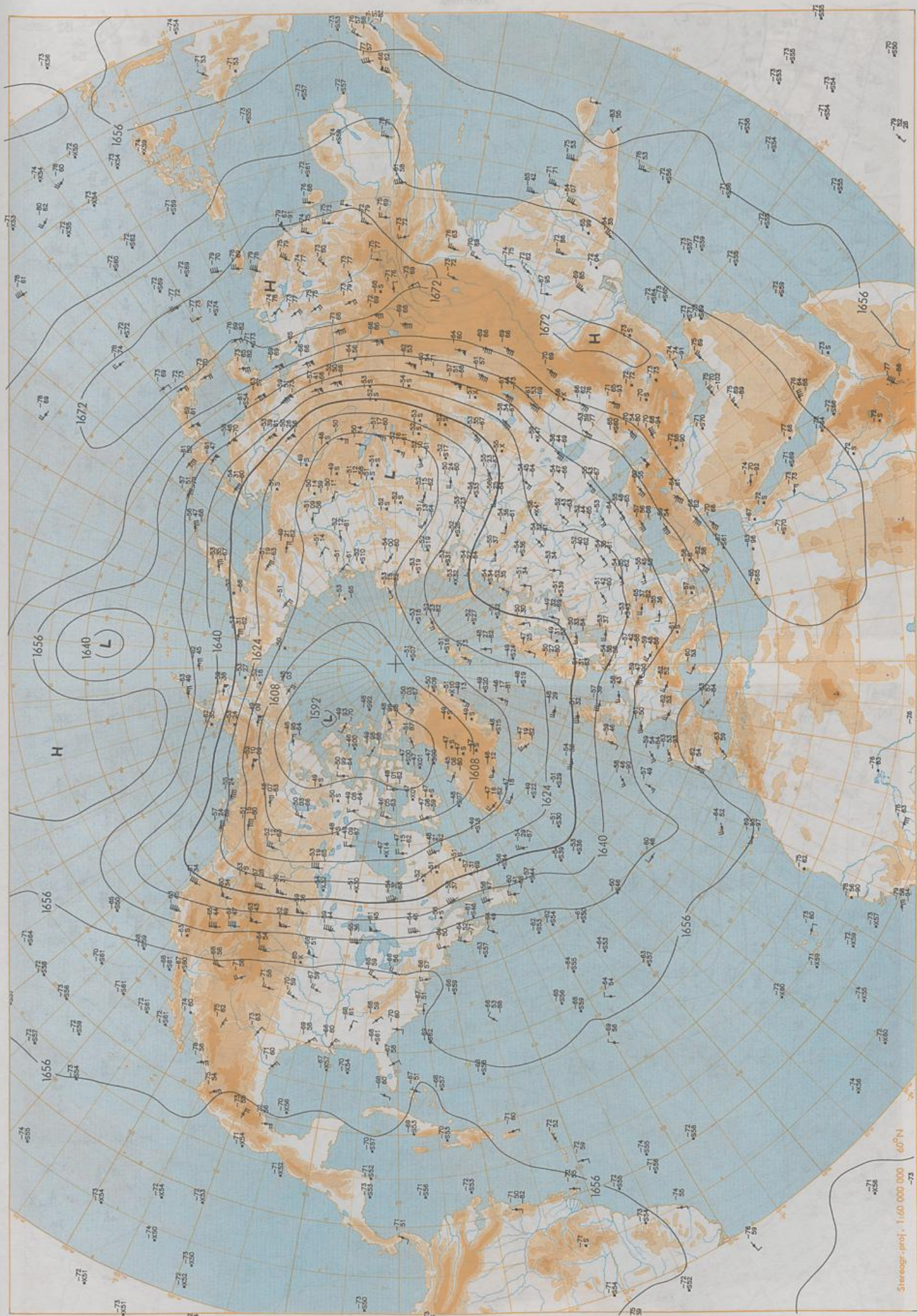
100 hPa 12 UTC
