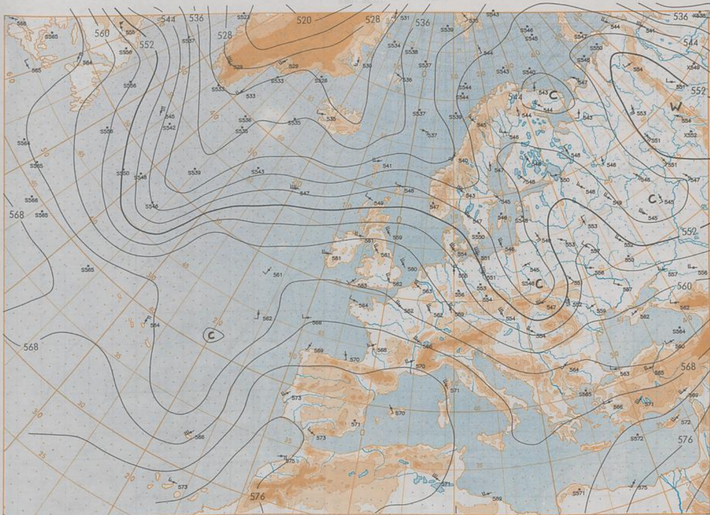
500/1000 hPa 12 UTC
