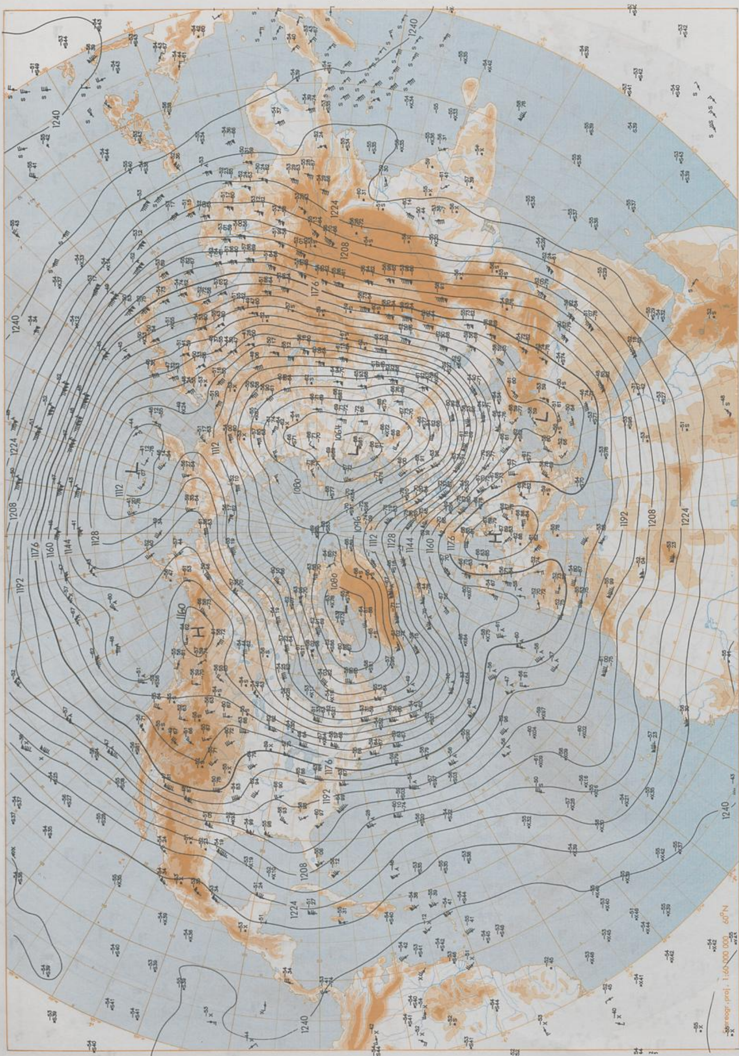
200 hPa 12 UTC
