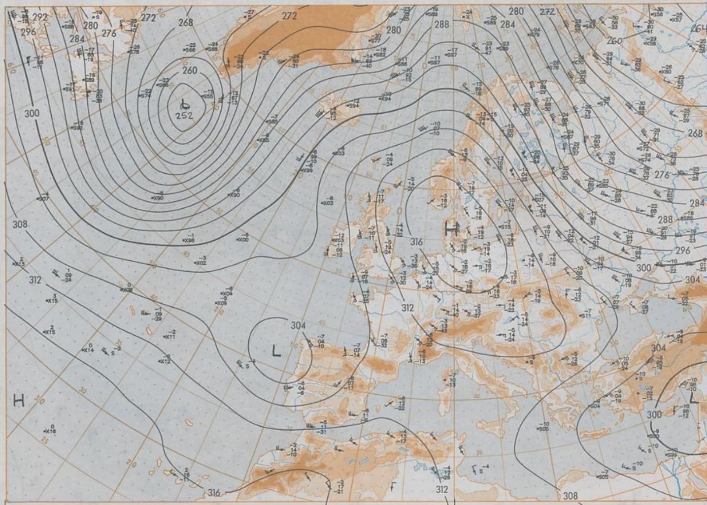
700 hPa 12 UTC
