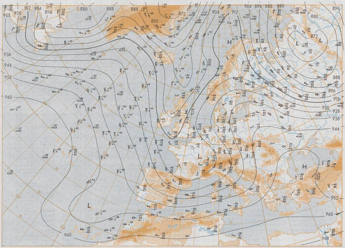
300 hPa 12 UTC
