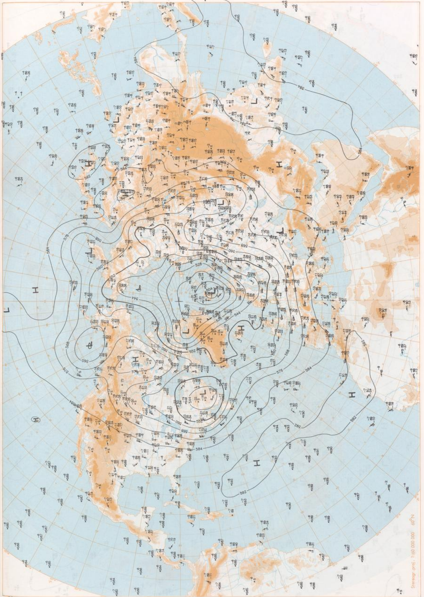
500 hPa 12 UTC
