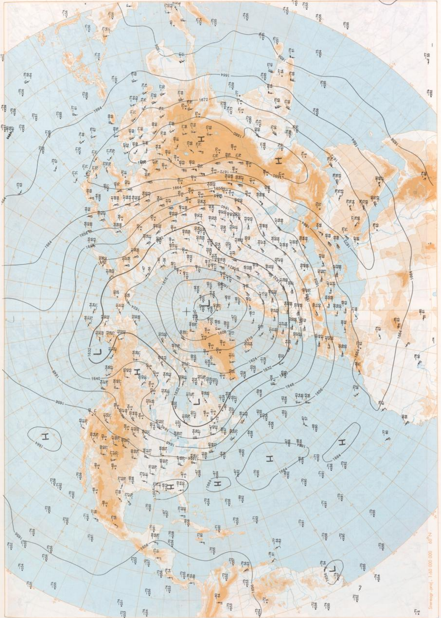
100 hPa 12 UTC
