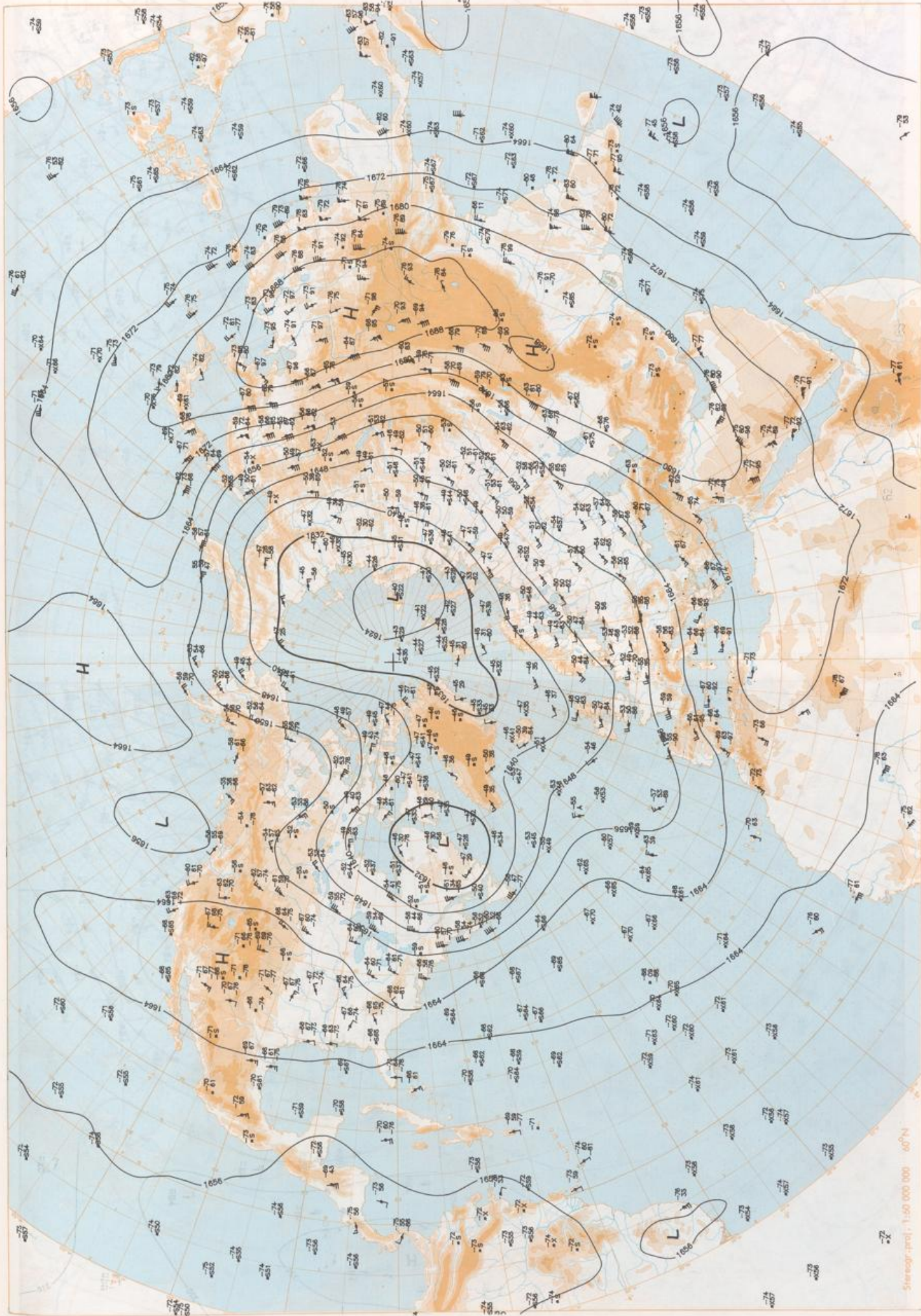
100 hPa 12 UTC
