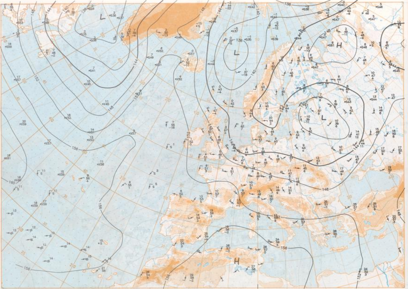
850 hPa 12 UTC
