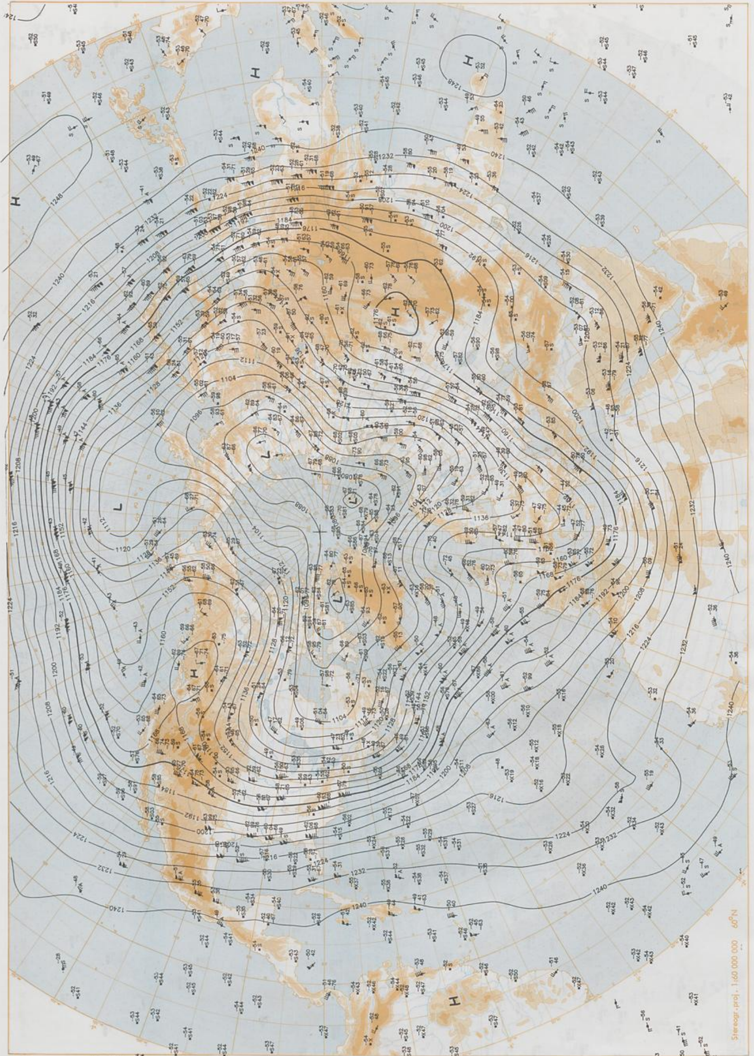
200 hPa 12 UTC
