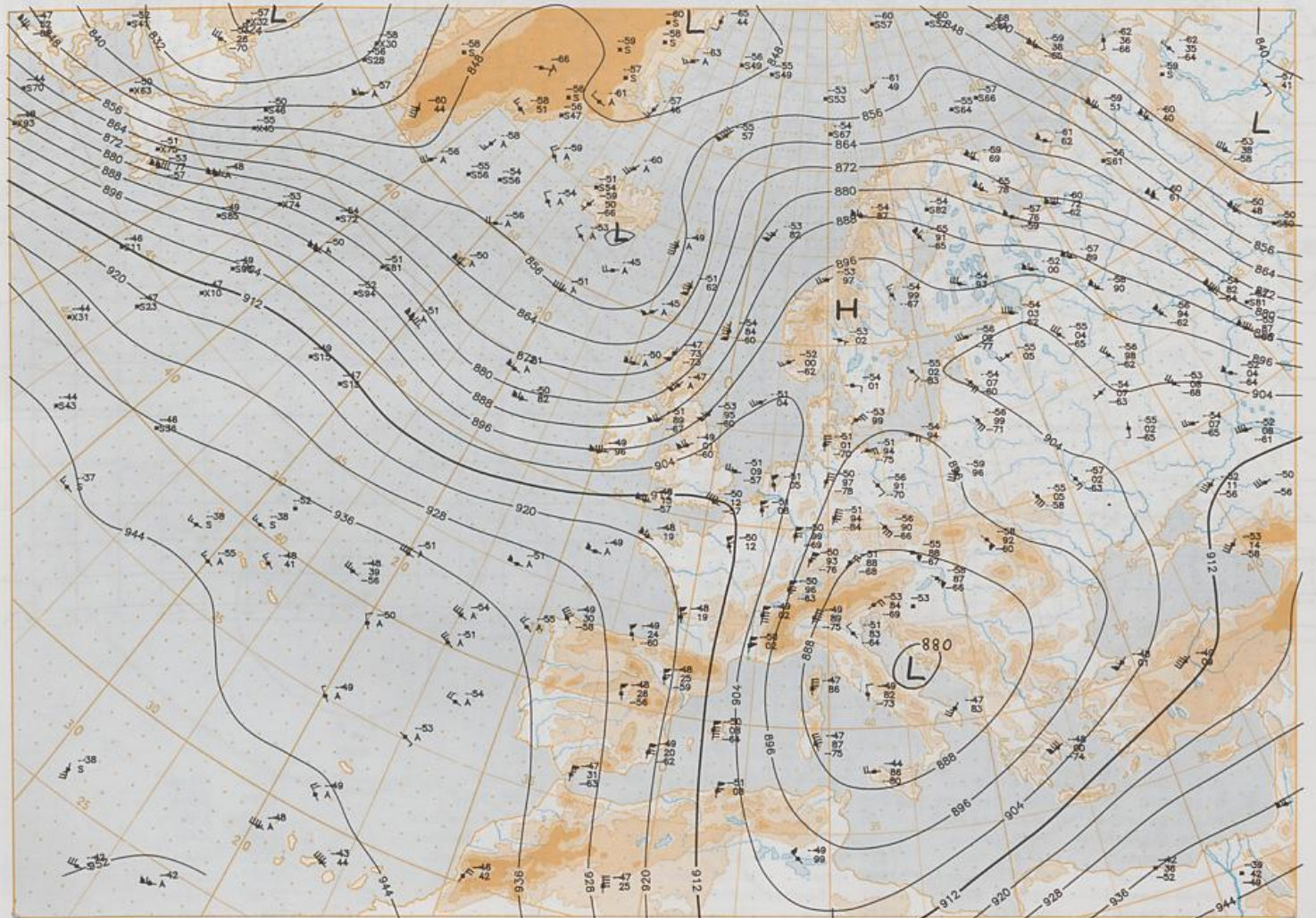
300 hPa 12 UTC
