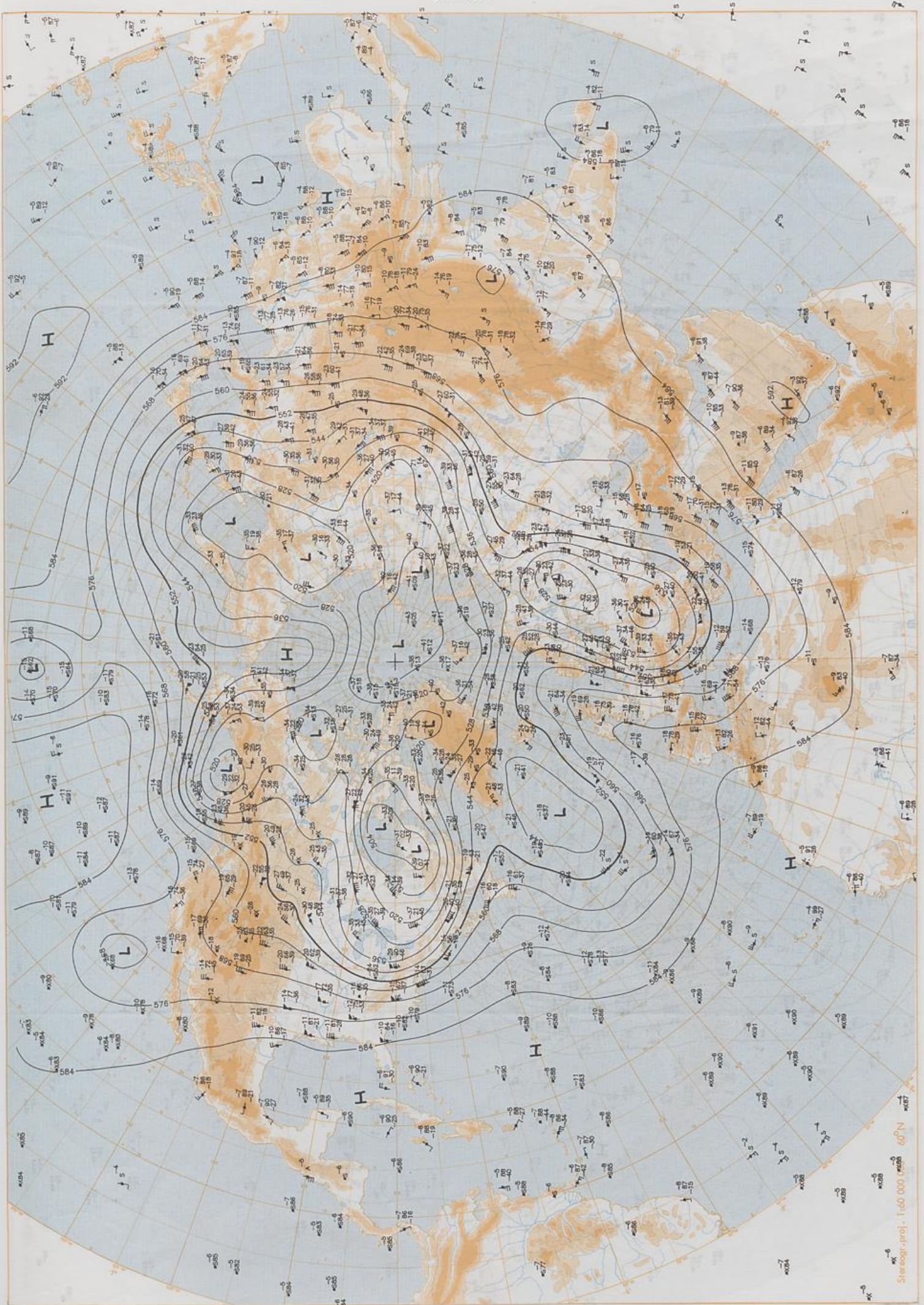
500 hPa 12 UTC
