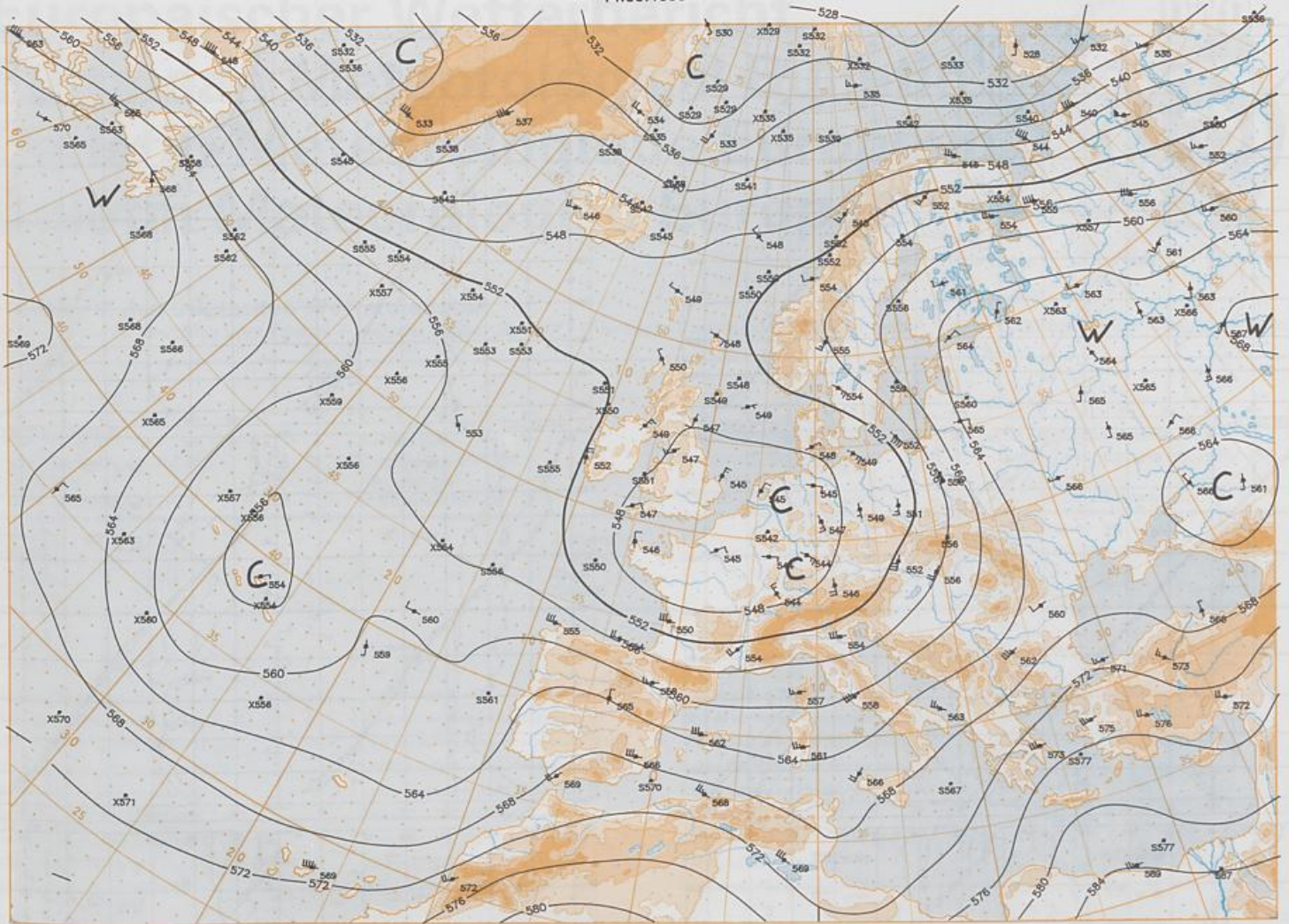
500/1000 hPa 12 UTC
