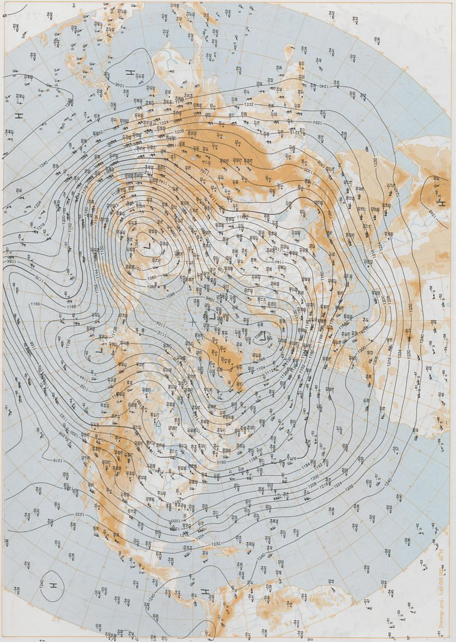
200 hPa 12 UTC
